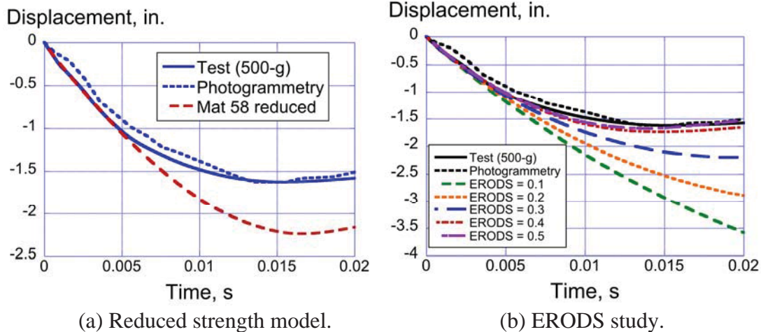
Figure 117. Mat 58 parameter study results for the cruciform section (268.6-in/s velocity).
