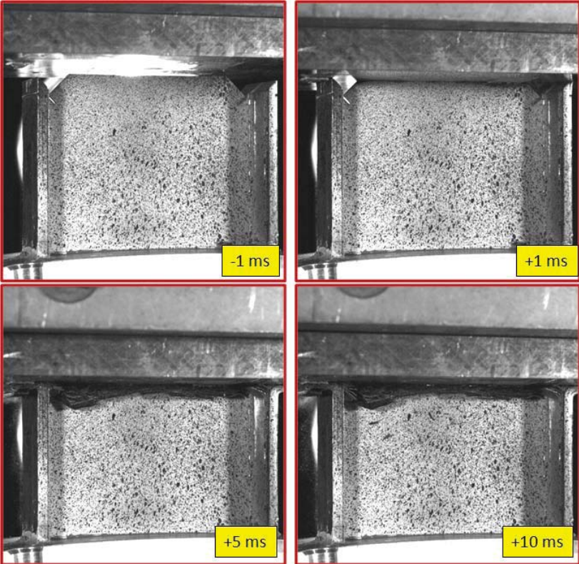
Figure 9. Image sequence of the I-beam 4-ft drop test.
