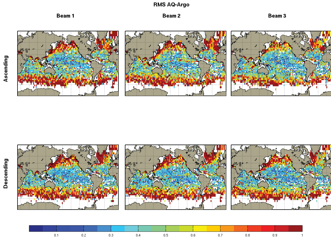
Figure 4. Same as Figure 3 but for the RMS difference between Aquarius SSS and bulk salinity from Argo.
