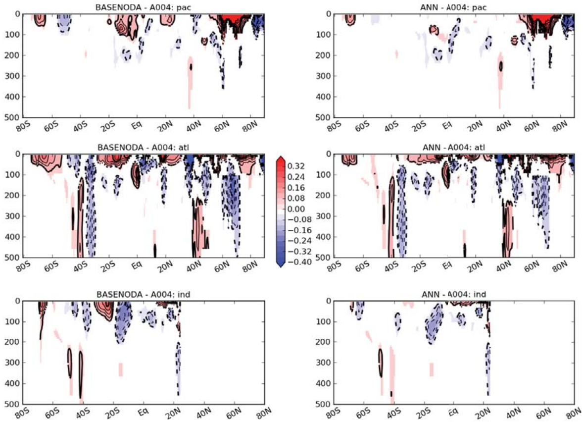
Figure 9. Climatologies of salinity of BASENODA minus MERRA-Ocean (left panels) and ANN minus MERRA-Ocean (right panels). From top to bottom, Pacific, Atlantic and Indian ocean.
