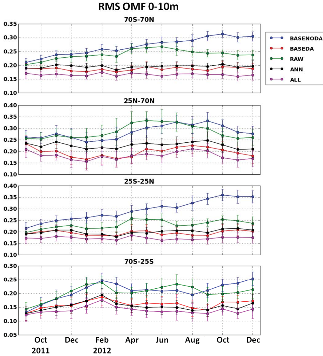
Figure 6. Time series of RMS of Argo bulk salinity minus a 1 day forecast from a prior analysis (OMF) in four latitude bands. From top to bottom: 70S to 70N, 25N to 70N, 25S to 25N and 70S to 25S.
