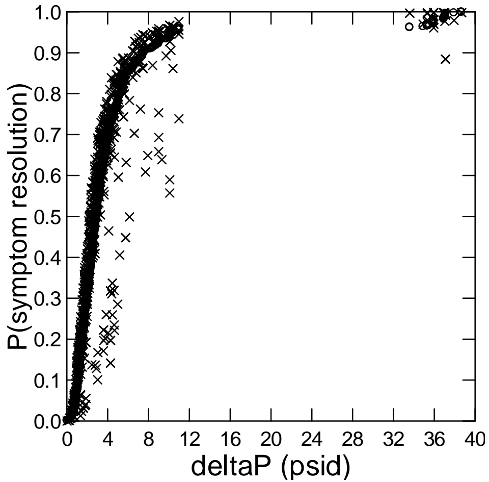
Fig. 48. The P(\text{symptom resolution}) with X-symbol compared to the empirical CDF [F_n(\Delta P)] of 831 symptoms with O-symbol from the validation set that resolved at the given \Delta P .
