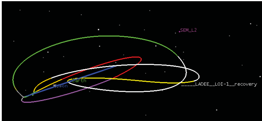
Figure 3: Contingency Trajectory Design for a missed LOI by the LADEE Spacecraft. Same trajectory as seen in Figure 1, except with a view edge-on the lunar orbit plane to show the out-of-plane components of the design. It is of note that a launch at a different time would have resulted in different forces (and thus different out-of-plane components) experienced by the spacecraft near the WSB region (to be discussed in the full paper).
