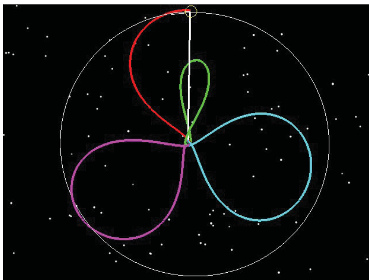
Figure 1: Nominal Trajectory Design for the LADEE Spacecraft. Earth-centered phasing loops are implemented to allow for launch window and launch insertion flexibility by the Minotaur V launch vehicle [1]
