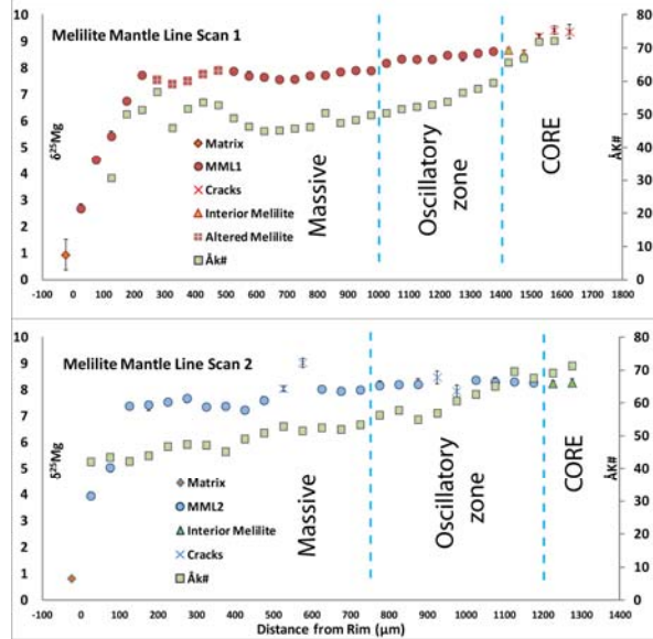
Figure 2 \delta^{25}\text{Mg} and \text{\AA}k_{\#} plotted vs. distance from rim. This is the complete transverse for both line scans. Cracks and obvious sections of alteration are indicated. The transitions between core, oscillatory zone and massive section are indicated with a dashed blue line. All error is reported as 2\sigma , much of the error is smaller than the data points.
