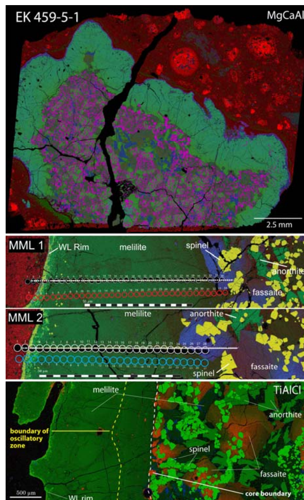
Figure 1. False colored qualitative 3 element x-ray maps. All labels are in RGB order (ex: MgCaAl; Mg-Red, Ca-Green, Al-Blue). (a) The entire studied grain, EK 459-5-1. (b) Both line scan transects across the melilite mantle, white line: EMPA transect, white open circles: trace element ablation pits, blue/red open circles: isotope spot locations. All open circles are 50 \mu\text{m} in diameter. Line scan localities relative to the whole grain can be seen in [7]. (c) X-ray map showing transitions between massive mantle, oscillatory zone and core-mantle boundary. Notice color change in melilite (darker, more åkermanitic melilite) as well as truncation of chlorine (blue) and Ti zoning in fassaite (edge of core vs. interior).
