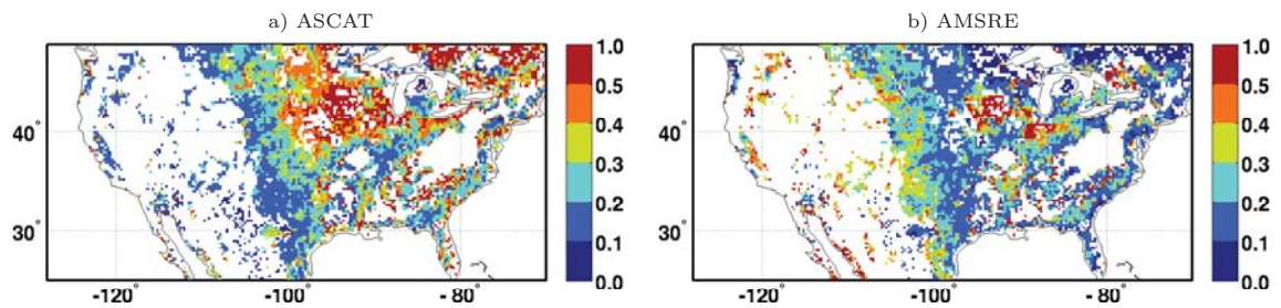
Figure 4: Width of the 90% confidence interval for the fRMSE TC of the a) ASCAT and b) AMSR-E soil moisture anomalies, plotted only where triple collocation results are available.
