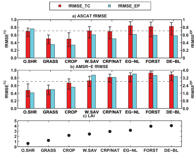
Figure 6: Mean by land cover class for the fRMSE^{TC} and fRMSE^{EP} of a) ASCAT and b) AMSR-E, and for c) LAI. For fRMSE^{TC} the 90% confidence interval is included (uncertainty estimates are not available for fRMSE^{EP} ). Note the different y-axis (on right) for the AMSR-E fRMSE^{EP} . The dashed line indicates a fRMSE of 1/\sqrt{2} , above which the signal to noise ratio is below one.
