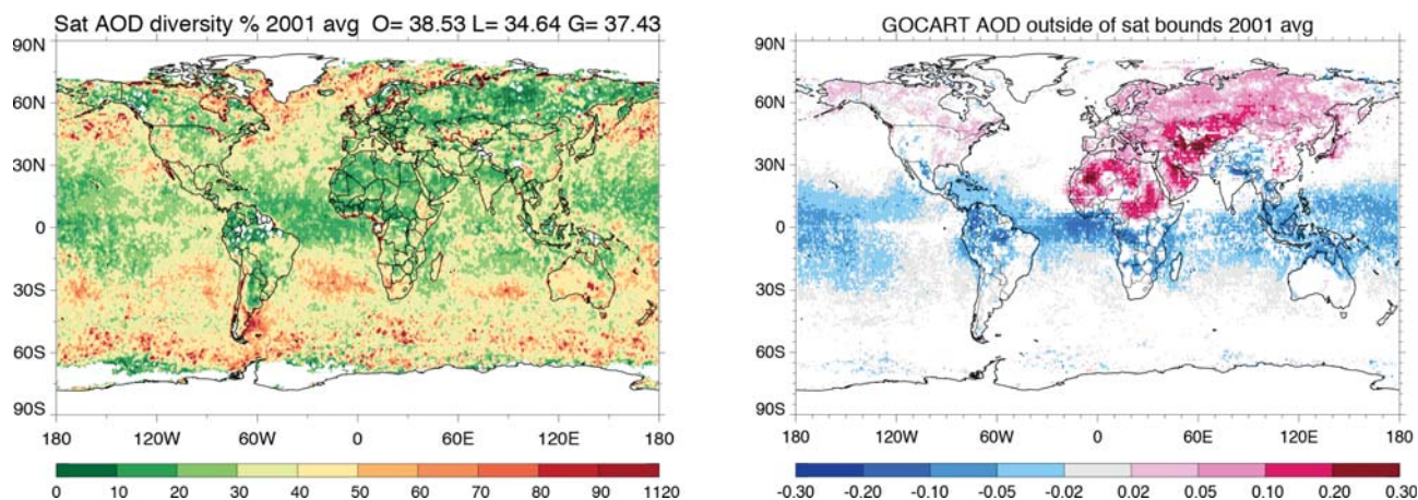
Fig. 5. (left) Satellite AOD diversity, defined as 1/2 (AOD_{\max} - AOD_{\min}) / AOD_{\text{median}} \times 100\% , for all available satellite annual mean AOD data points shown in Fig. 4, and (right) GOCART-simulated AOD that are outside of the satellite AOD range.
