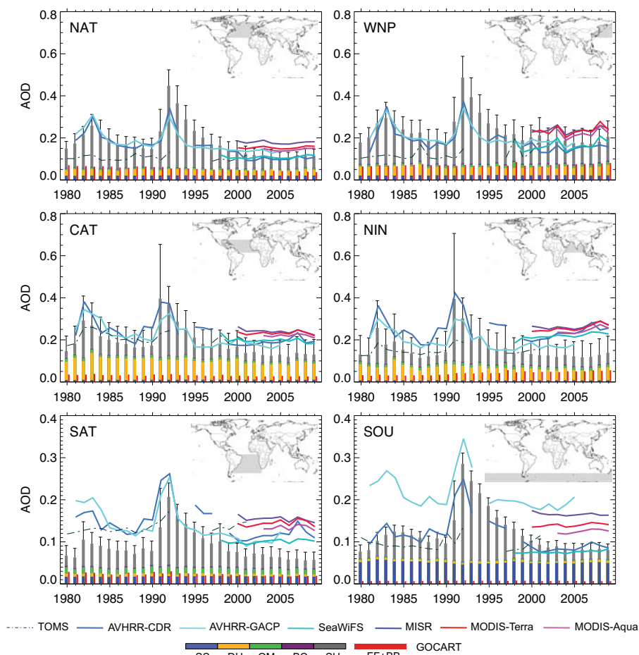
Fig. 9. Same as Fig. 6a but for six ocean regions of NAT, CAT, SAT, WNP, NIN, and SOU (domains shaded in grey). AVHRR retrievals are available over ocean.
