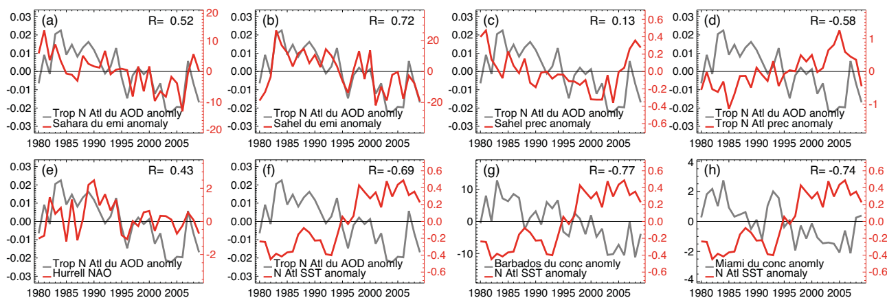
Fig. 14. From (a) to (e): time series of GOCART-calculated tropical North Atlantic ( 5\text{--}20^\circ\text{N} , 90\text{--}18^\circ\text{W} ) dust AOD anomaly (dark grey line) vs. (red line) model-calculated Sahara dust emission anomaly (a), model-calculated Sahel dust emission anomaly (b), MERRA Sahel precipitation anomaly (c), MERRA tropical North Atlantic precipitation anomaly (d), Hurrell principle component-based NAO index ( http://climatedataguide.ucar.edu/guidance/hurrell-north-atlantic-oscillation-nao-index-pc-based ) (e), and MERRA North Atlantic ( 0\text{--}66^\circ\text{N} ) SST anomaly (f). From (g) to (h): time series of GOCART-calculated Barbados (g) and Miami (h) dust concentration anomaly vs. North Atlantic SST anomaly. Anomaly is defined as the difference between the annual average value and the 30-year mean.
