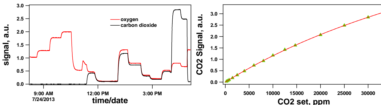
Figure 11. Carbon dioxide calibration step challenges and calibration. The Multi-Gas Monitor was simultaneously calibrated with step challenges of oxygen and carbon dioxide. At high concentrations curvature is evident in the fit against concentration but is easily accommodated by the fitting algorithm.
