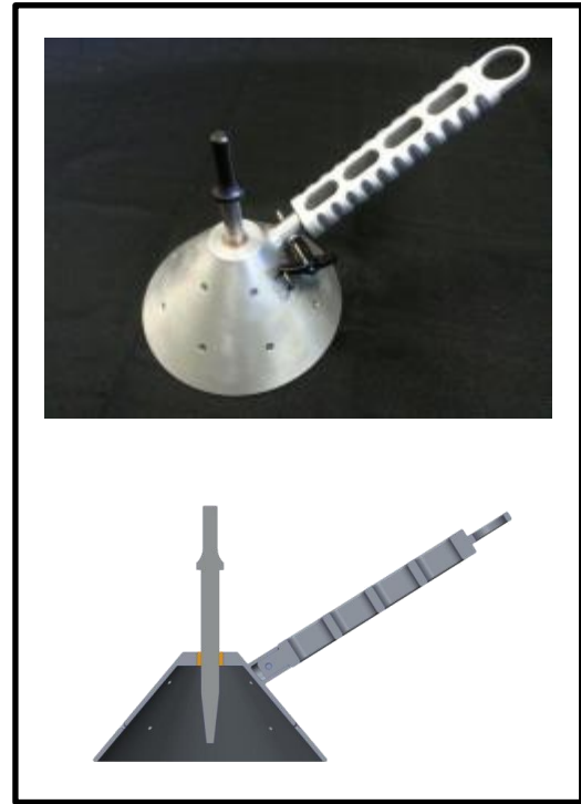
Figure 7 EVA Geology – “Hammer Sampling Cup”
