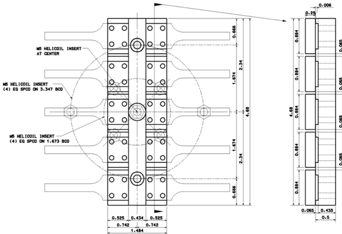
Figure 30.—Ten-specimen fixture arrangement on shaker armature (all dimensions shown in inches).
