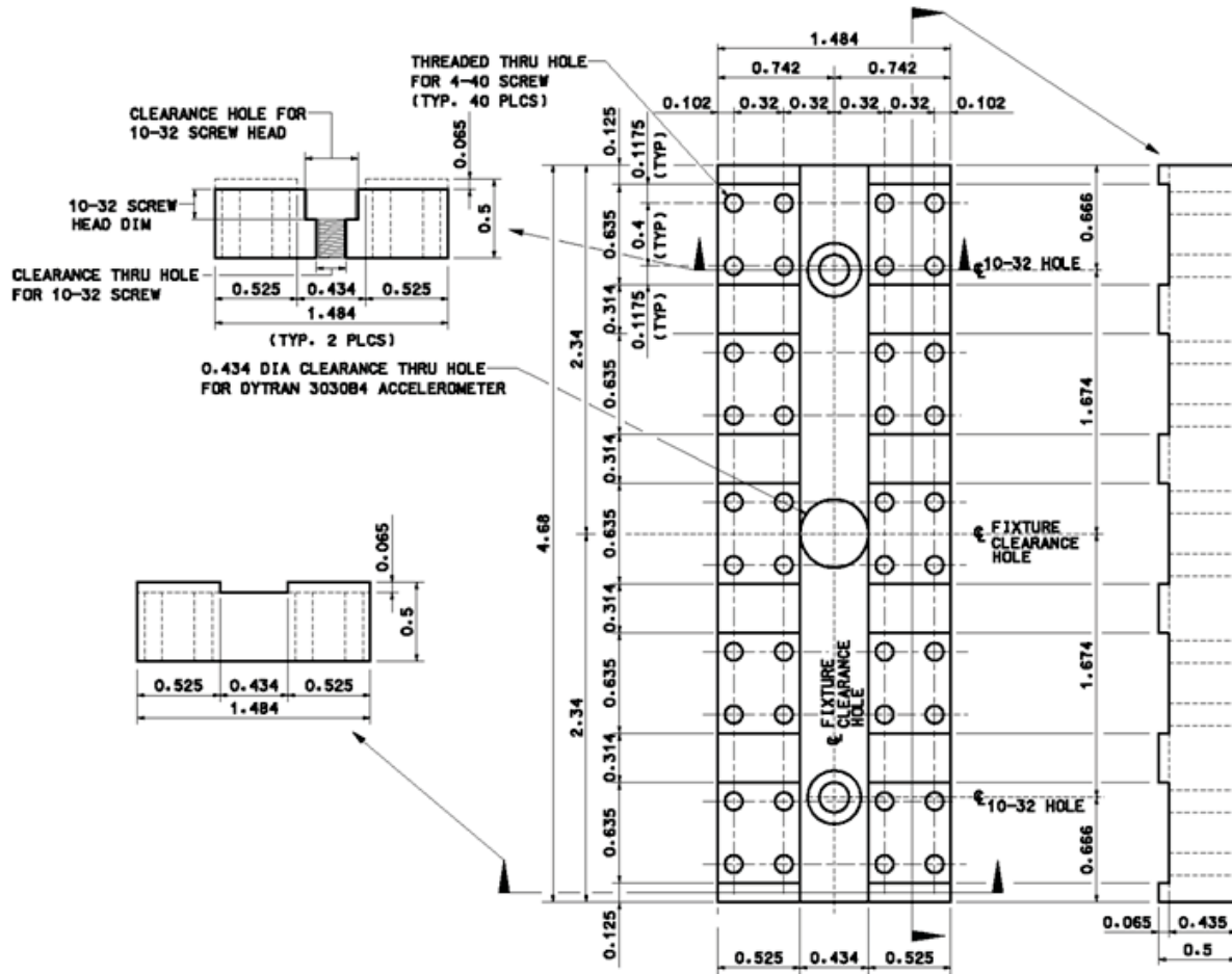
Figure 29.—Drawing of lower block for 10-specimen fixture (all dimensions shown in inches).
