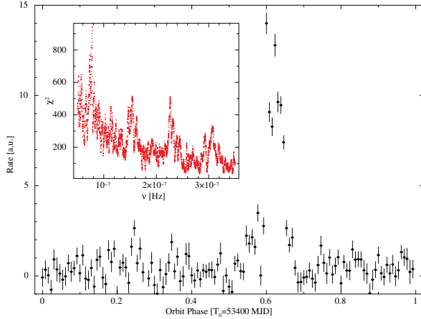
Fig. 2. Folded Swift /BAT light curve (15–150 keV) of RXJ0440.9+4431 at the best determined orbital period, (150.0 \pm 0.2) days. The inset shows the periodogram obtained from the epoch folding technique applied to the Swift /BAT light curve.
