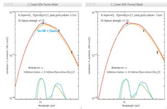
Figure 3: Better-fit thermal models for comet ISON at r_h \approx 1.2 AU, for a_p=0.7 \mu\text{m} (left) and a_p=1.0 \mu\text{m} (right), porosity parameter D=2.7 and slope N=4.5 . Models are fitted to three FORCAST photometry points (black points with error bars, and constrained by the silicate feature strength \leq 1.1 and the N-band continuum color temperature of T_{bb}=260\text{--}265 \text{ K} [15] (blue dashed line of a graybody at this temperature). Mineralogy is amorphous carbon-to-amorphous silicate ratio = 9, with amorphous carbon (orange), amorphous pyroxene, amorphous olivine (green), and the total SED (red).
