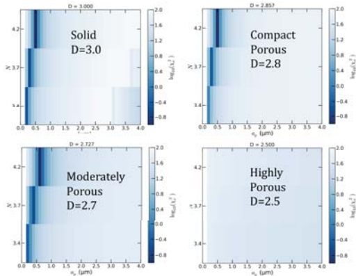
Figure 2: Reduced \chi_r^2 for thermal models fitted to three FORCAST photometry points and with the constraint that the silicate feature strength \leq 1.1 for comet ISON at r_h \approx 1.2 AU.
