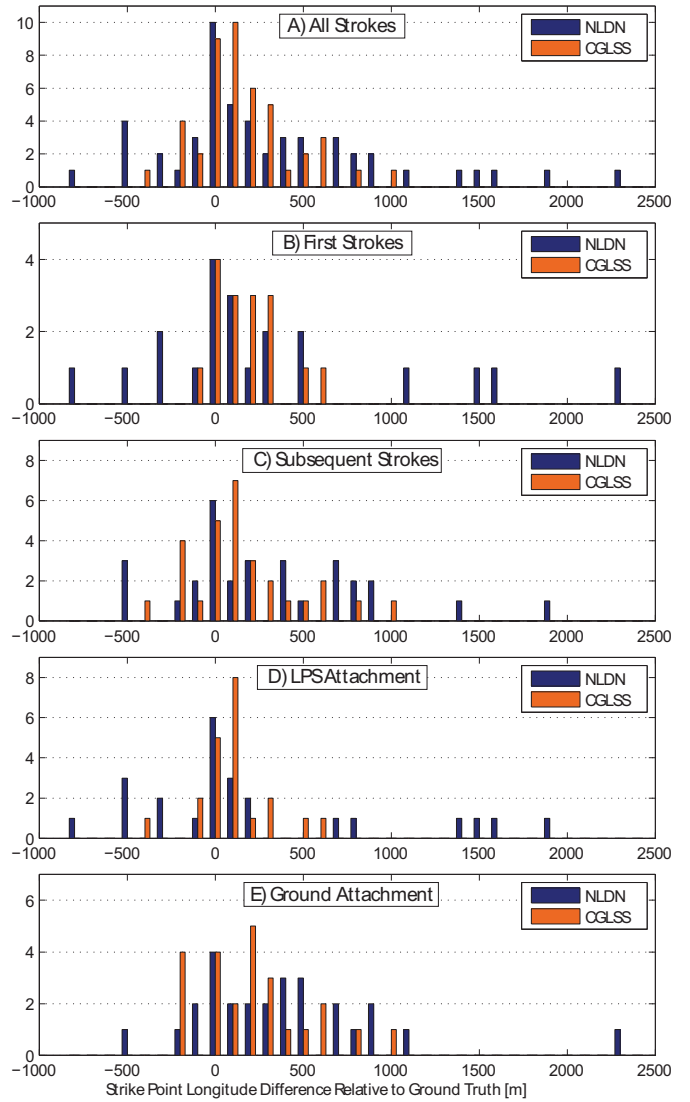
Fig 3. Distributions of longitudinal strike point location differences of NLDN and CGLSS systems relative to ground truth.
