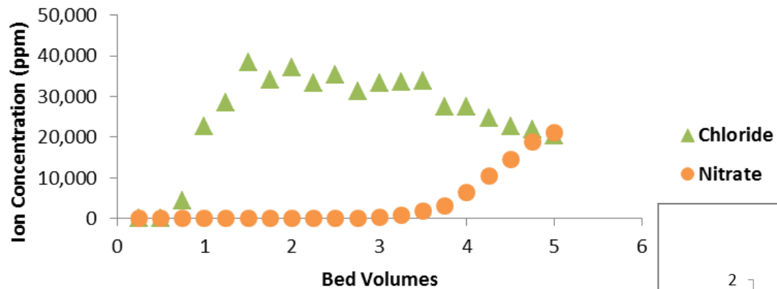
IRA900 Resin Selectivity Run
