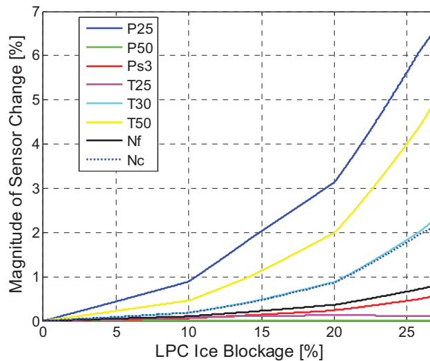
Figure 4.—Magnitude of the change in sensor output for all sensors in the C-MAPSS40k engine as the size of the ice blockage in the LPC increases. This data is collected at 10,000 ft, Mach 0.6, and a PLA of 68°.
