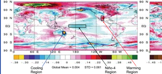
AIRS T_{skin} ARC (K/yr) September 2002 through August 2013 1:30 AM/1:30 PM Average
