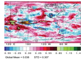
AIRS Cloud Fraction ARC (%/yr) September 2002 through August 2013 1:30 AM/1:30 PM Average
