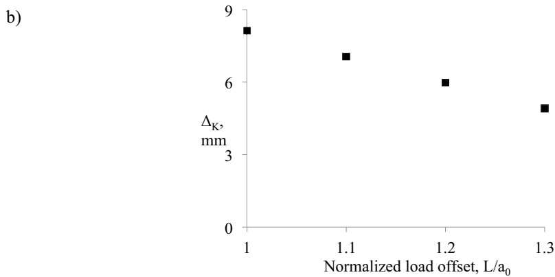
Figure 11(a) typical crack path, (b) distance from the migration location to the load-application point, \Delta_K , as a function of load-offset L .
