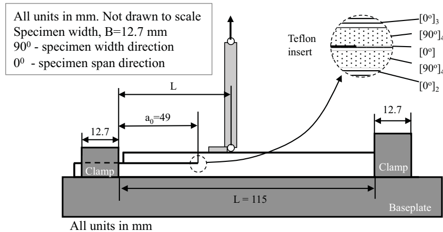
Figure 7 Delamination Migration (DM) test configuration [8].
