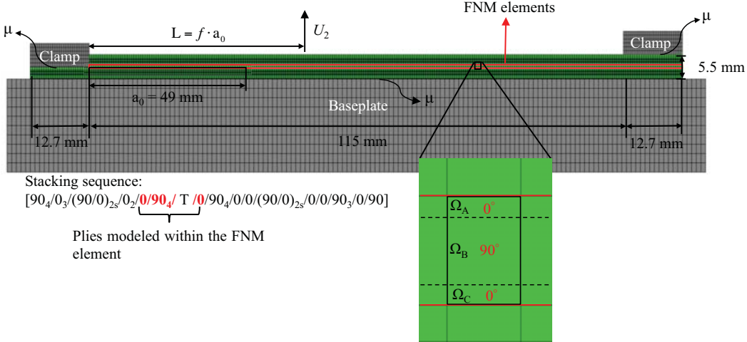
Figure 8 Finite element model used.
