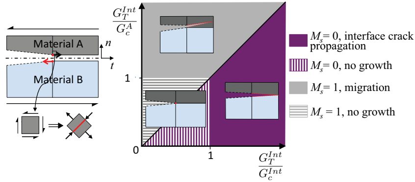
b) negative shear
