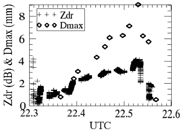
Fig. 3: Z_{dr} extracted over the 2DVD site (after smoothing in range) as time series from the CHILL radar fixed pointing measurements and D_{max} recorded by the 2DVD at ground level.
