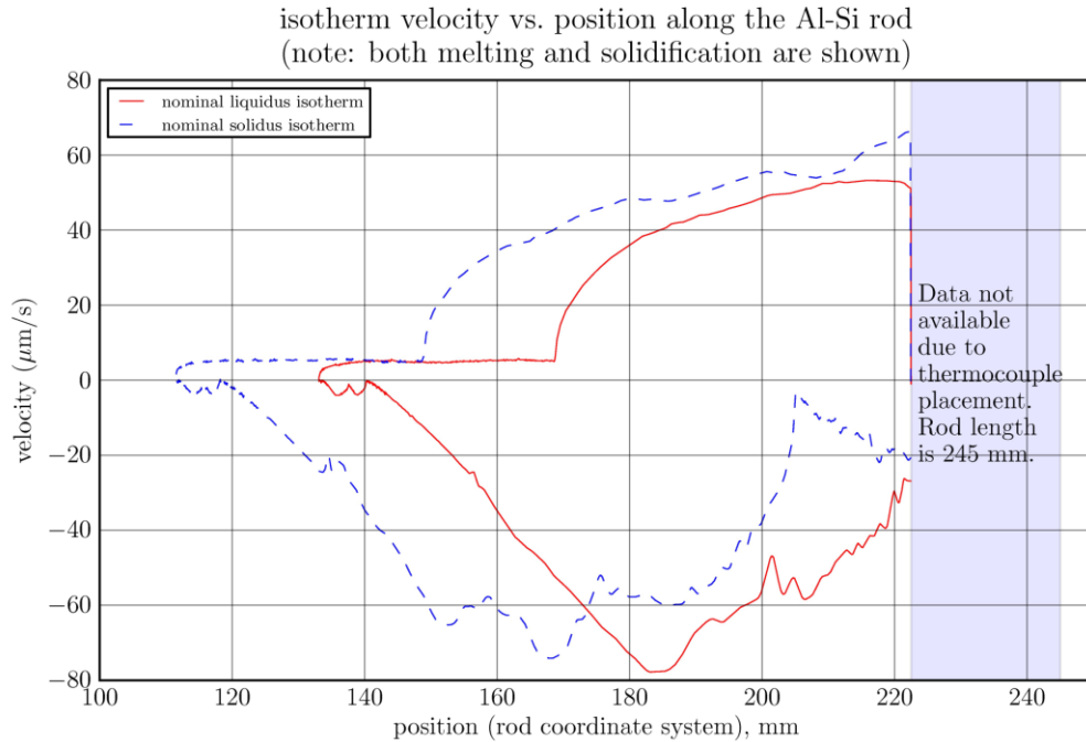
Figure 6: Liquidus-isotherm velocity (solid red curve) and solidus-isotherm velocity (broken blue curve) for MICAST6. Pre-DS has the negative velocities; the DS has positive velocities. The DS withdrawal rate was 5 \mu\text{m s}^{-1} for 3.8 cm and 50 \mu\text{m s}^{-1} for 11.3 cm.
