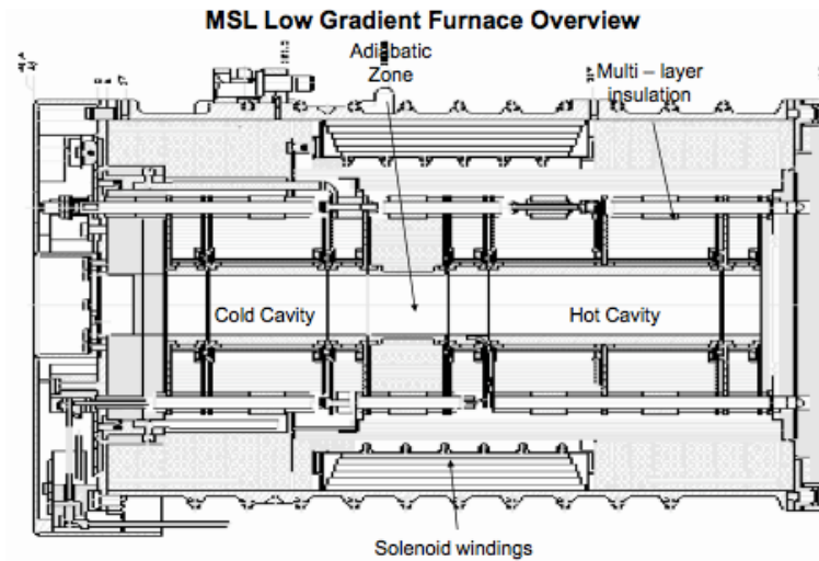
Figure 2: Schematic of Low Gradient Furnace (LGF) used for the directional solidification of MICAST6.
