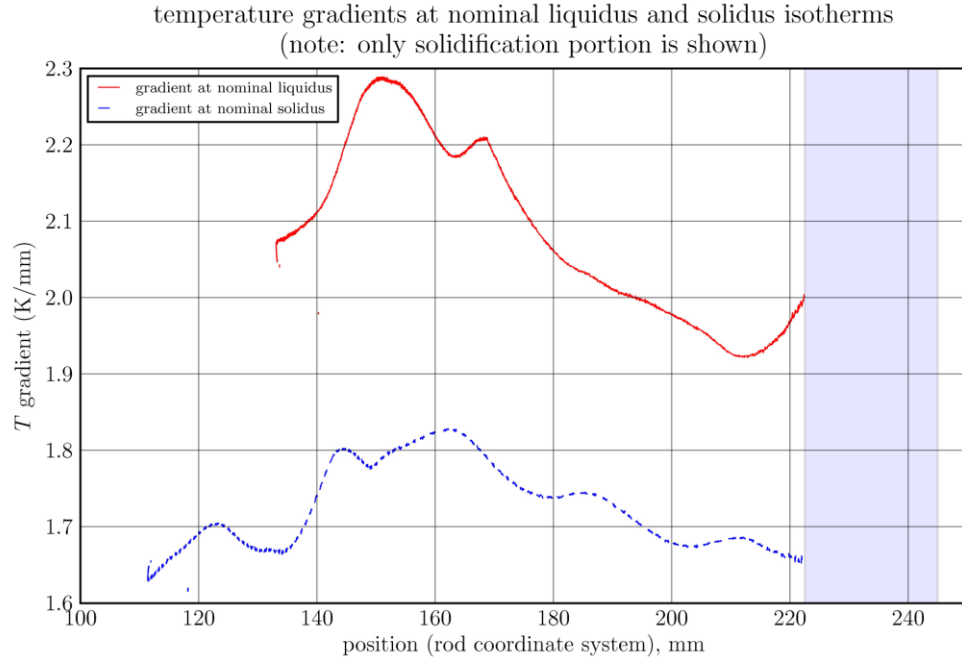
Figure 7: Thermal gradient at liquidus (red curve) and at eutectic-solidus (blue curve) for MICAST6. DS withdrawal rate 5 \mu\text{m s}^{-1} for 3.8 cm and 50 \mu\text{m s}^{-1} for 11.3 cm
