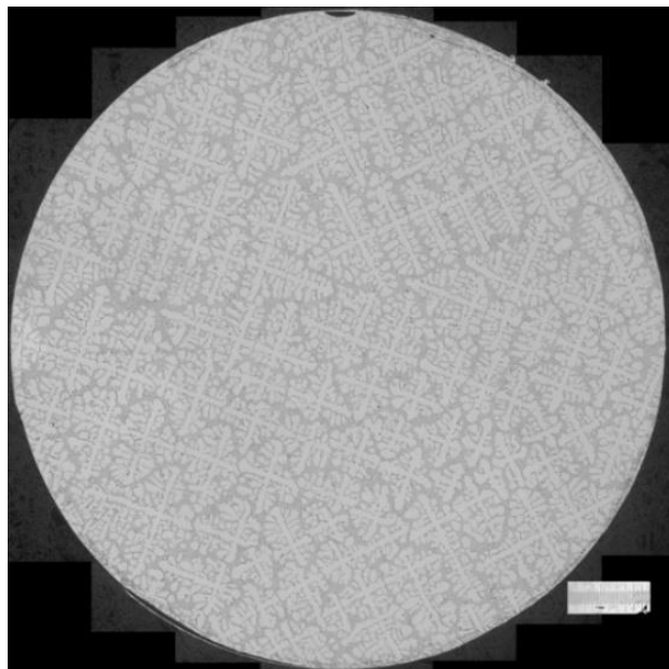
Figure 5: Transverse section of a crystal made at CSU with a solidification velocity of 22 \mu\text{m s}^{-1} in a thermal gradient of 41 \text{ }^\circ\text{C cm}^{-1} . This sample was used as the seed crystal for MICAST6.
