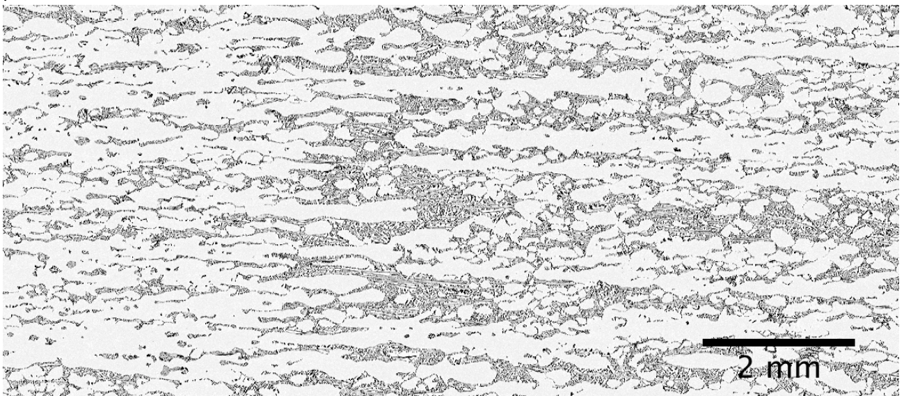
Figure 14: EMPA X-ray map of Si in MICAST6 at the end of the pre-DS mushy zone.
