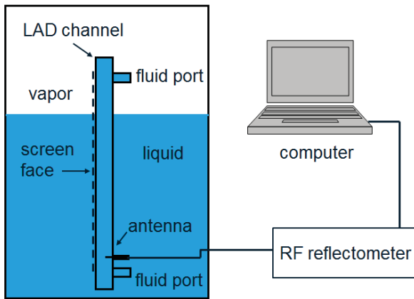
Figure 2. Schematic of the test setup used for RF measurements of liquid quantity in the LAD channel.
