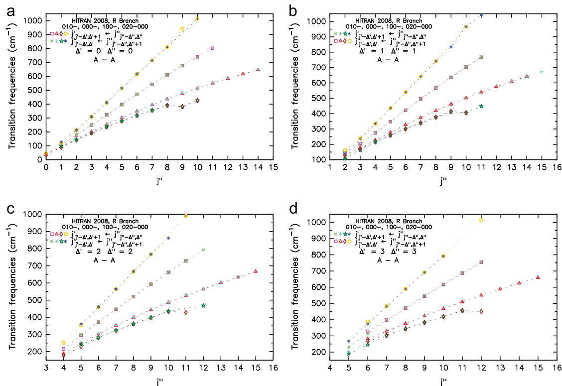
Fig. 1. The screening results of the transition frequency for the four groups of j''_{j'-\Delta',\Delta''+1} \leftarrow j''_{j'-\Delta',\Delta''} and j''_{j'-\Delta',\Delta''+1} \leftarrow j''_{j'-\Delta',\Delta''+1} in the R branch associated with the four selections of \Delta' and \Delta'' in the 010–000, 000–000, 100–000, and 020–000 bands. The transition frequencies of these pairs subtracted by the band center in the four bands are plotted by \{\square, \times\} , \{\triangle, +\} , \{\diamond, \star\} , and \{\circ, *\} , respectively, in Fig. 1(a)–(d).
