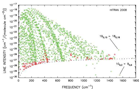
Fig. 14. The distribution of 81 missing H 2 O lines in the pure rotational band over the transition positions. Their predicted intensities (in cm -1 / (molecule cm -2 )) are plotted by \Delta . The original 1639 H 2 O lines listed in HITRAN 2008 are also plotted by \times . The intensity threshold is plotted by a dotted line.
