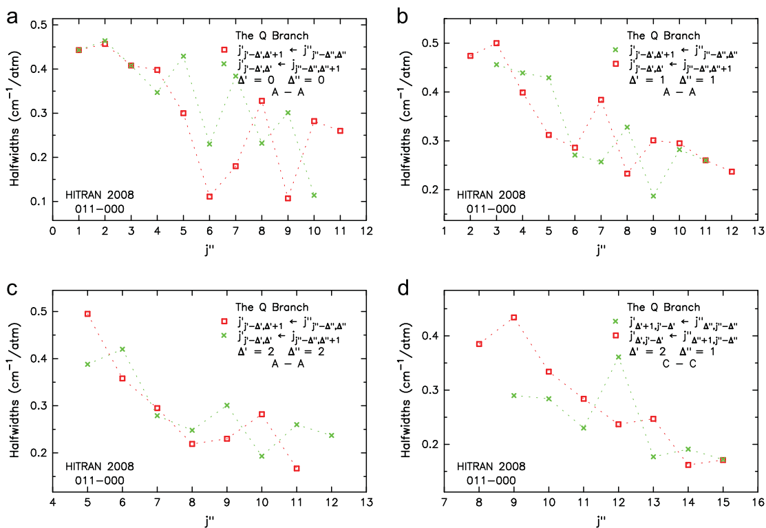
Fig. 10. The same as Fig. 9 except for self-broadened half-widths associated with four specified groups in the Q branch of the 011–000 band.
