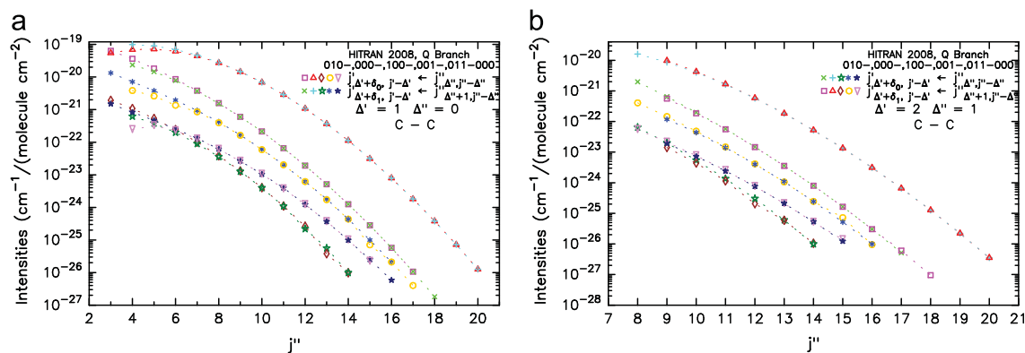
Fig. 3. The intensities of paired lines (in \text{cm}^{-1}/(\text{molecule cm}^{-2}) ) in two groups in the C–C case and in the Q branch, and with \Delta' = 1 , \Delta'' = 0 and \Delta' = 2 , \Delta'' = 1 , respectively, in the five important \text{H}_2\text{O} bands labeled by 000–000, 010–000, 100–000, 001–000, and 011–000 are plotted in Fig. 3(a) and (b). By excluding the spin degeneracy factor, for each of the two paired lines, their intensity values in the five bands listed in HITRAN 2008 are represented by five different symbols. In addition, the same symbols are connected by their corresponding lines.
