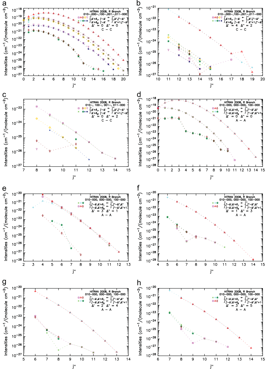
Fig. 4. The same as Fig. 3 except for the eight specified groups of lines whose intensities are plotted Fig. 4(a)–(h). In addition, these eight groups are not always available in all the five bands. In case the groups of interest become unavailable in some bands, the corresponding symbols and labels are absent in the plotting.
