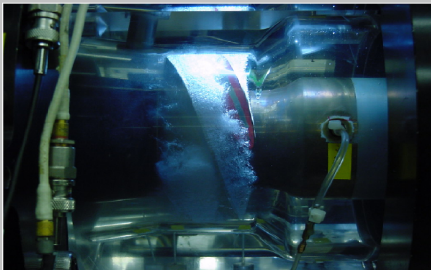
RS-25 High-Pressure Lox Inducer in Waterflow Test at MSFC
