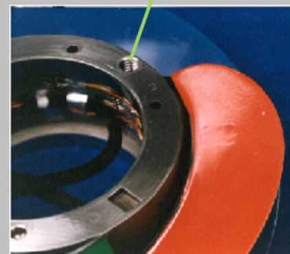
Instrumented RS-25 High-Pressure Lox Inducer
