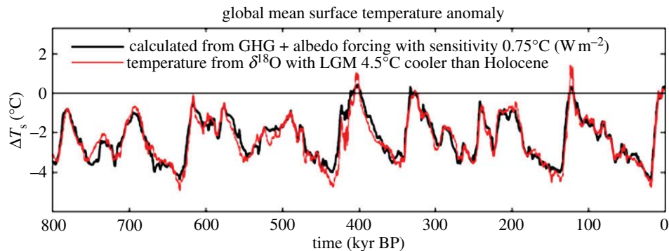
Figure 6. Calculated surface temperature for forcings of figure 5c with a climate sensitivity of 0.75°C per W m -2 , compared with 2 \times \Delta T_{\text{do}} . Zero point is the Holocene (10 kyr) mean.
