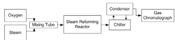
Fig. 7: KSC Steam-Reformer System Flow Diagram.
