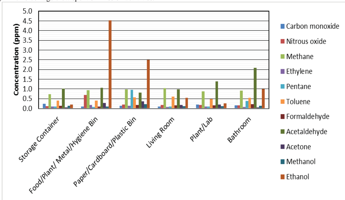
Fig. 123: Average concentrations of selected VOCs at different habitat locations during the first 60 days of the mission.
