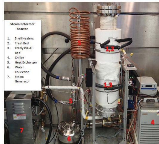
Fig. 8: KSC Steam Reforming Reactor System.
