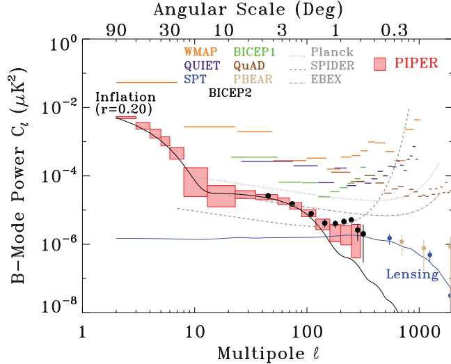
Figure 2: The B-mode power spectrum assuming a tensor-to-scalar ratio r = 0.2 from inflationary gravitational waves and gravitational lensing. The quantity being measured C_{\ell}^{\text{BB}} is plotted, rather than \ell(\ell + 1)C_{\ell}^{\text{BB}}/2\pi . Theories of inflation generically predict a rise in power at \ell < 10 . PIPER will measure the shape of the spectrum for 2 \leq \ell < 300 , encompassing the “reionization bump” at low \ell , the “recombination bump” at \ell \sim 80 , as well as the lensing signal at \ell > 200 .
