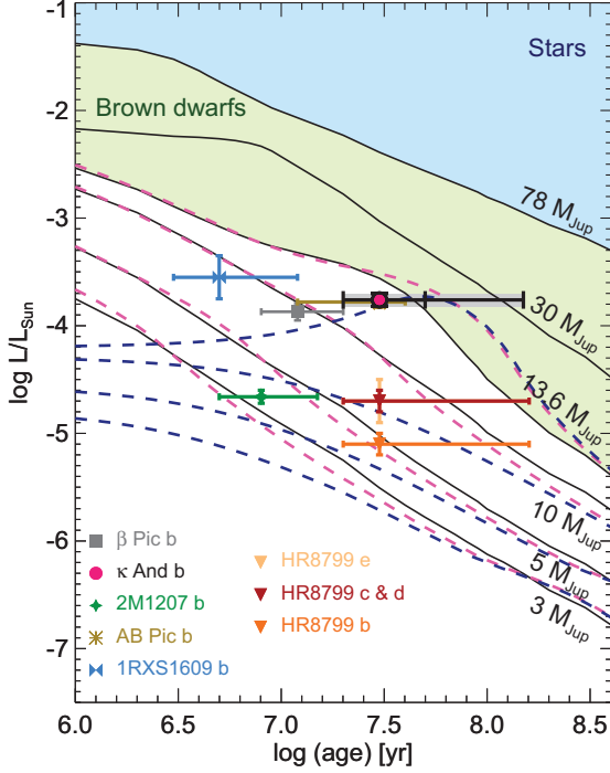
Fig. 10. Evolution of the luminosity of gaseous objects predicted by the COND models (black solid line), and Marleau & Cumming (2013) models with typical “hot-start” (light pink dashed curve; 3, 5, 10, 13.6 M_{\text{Jup}} ), and “cold-start” initial conditions (dark blue dashed curve; 3, 5, 10, 13.6 M_{\text{Jup}} ). We overlay measured luminosity of young low mass companions. A more complete version of this figure can be found in Marleau & Cumming (2013).
