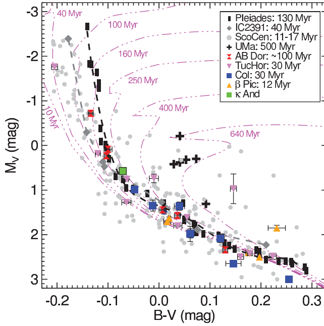
Fig. 3. Position of \kappa And A in a color-magnitude diagram (CMD) compared to other A and B-type member of the Pleiades, the IC 2391 cluster, Scorpius-Centaurus (ScoCen), Ursa Majoris group, and other young moving groups in the solar neighborhood (see legend). The star’s position in the diagram is consistent with some members of all the plotted samples except the Ursa Majoris moving group (UMa), which is clearly older and more evolved. The placement in the CMD suggests that \kappa And is not much older than the upper limit of the Pleiades, 150 Myr. The dashed-dotted lines are Ekström et al. (2012) tracks that include rotation. These models predict an age of \lesssim 250 Myr for \kappa And, but they overestimate the ages of B-type cluster members. The dotted lines are 5th order polynomial fits to the Pleiades and IC 2391 sequences and are shown to highlight them for clarity.
