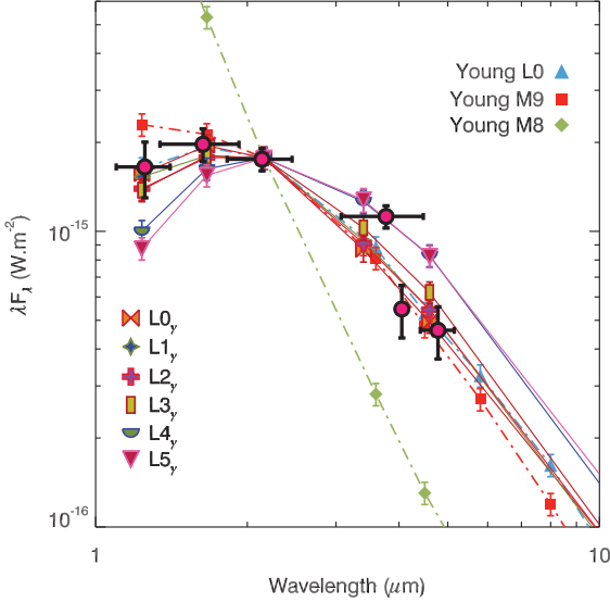
Fig. 7. \kappa And b spectral energy distribution (magenta dots) compared to the mean spectral energy distribution of young M8-L0 dwarfs (Luhman et al. 2010) and of L0-L5 _{\gamma} dwarfs (Faherty et al. 2013).
