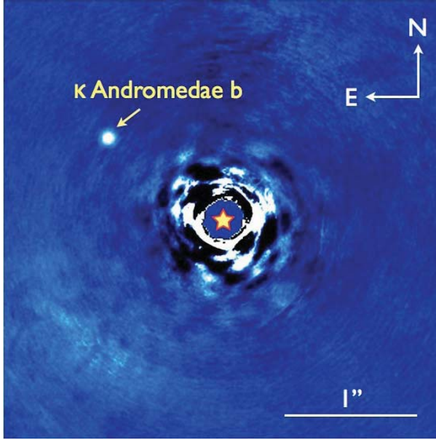
Fig. 2. LBTI/LMIRCam high-contrast image of the \kappa And system at M band. The companion is recovered.
