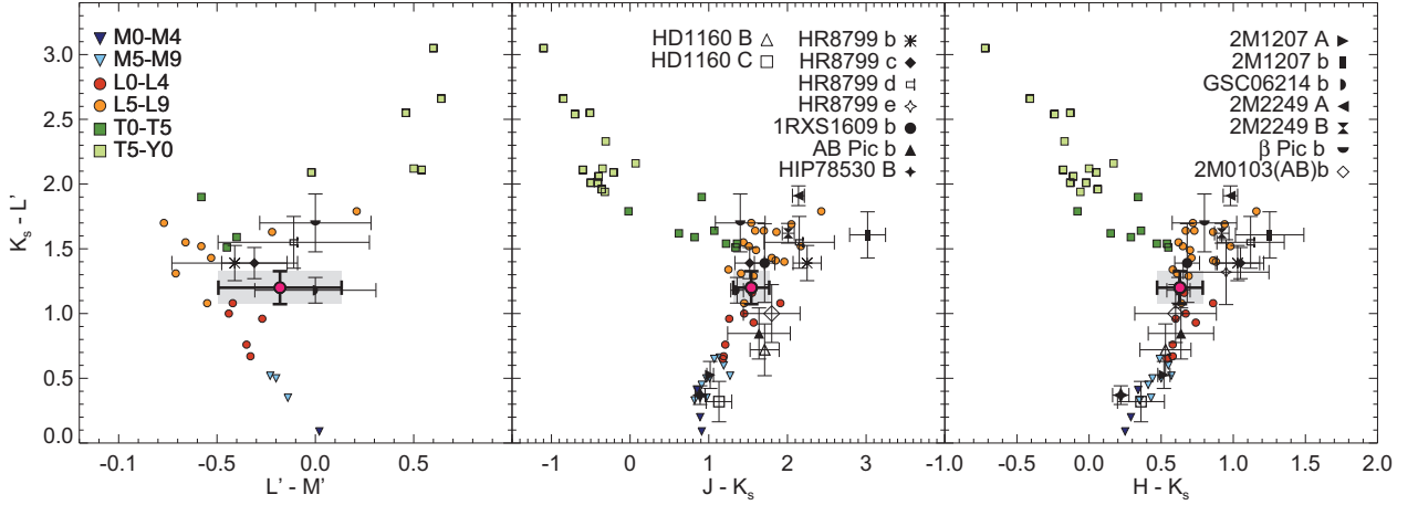
Fig. 5. \kappa And b (magenta dot) in color-color diagrams compared to known MLTY field dwarfs and brown-dwarfs, and young directly imaged companions. The photometry of young companions is referenced in Bonnefoy et al. (2013a,b) (and ref. therein), Nielsen et al. (2012), and Delorme et al. (2013). The photometry of MLTY field dwarfs is taken from Leggett et al. (2010, 2013).
