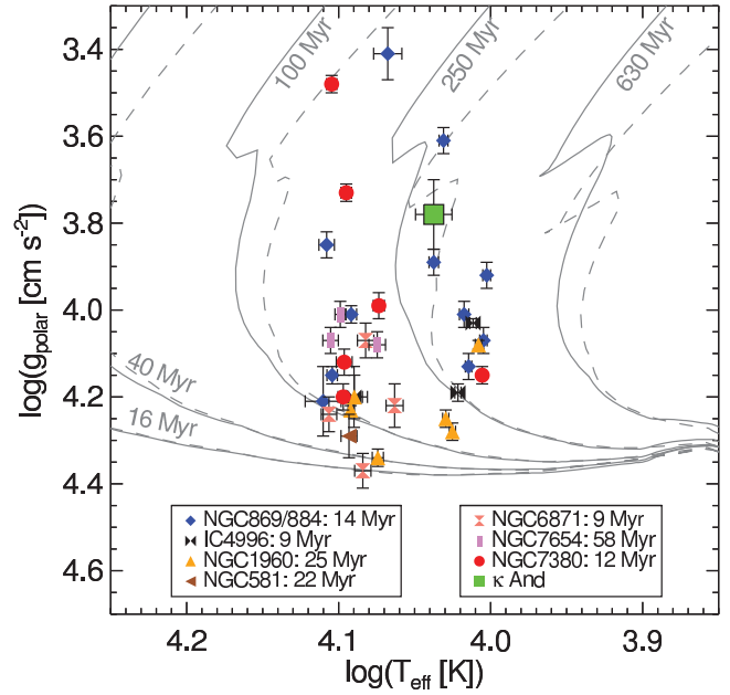
Fig. 4. Position of \kappa And A in a temperature-gravity diagram compared to the models of Ekström et al. (2012) for rotating (solid lines; V/V_{crit} = 0.4 when stars reach the zero-age main-sequence) and non-rotating (dashed lines). We also show the same parameters for similarly typed members of young clusters (see legend). The models do not reproduce the ages of the cluster members and there is significant scatter in the polar gravity estimates within a given cluster. We interpret this as indication that these comparisons do not place a meaningful constraint on the age of \kappa And.
