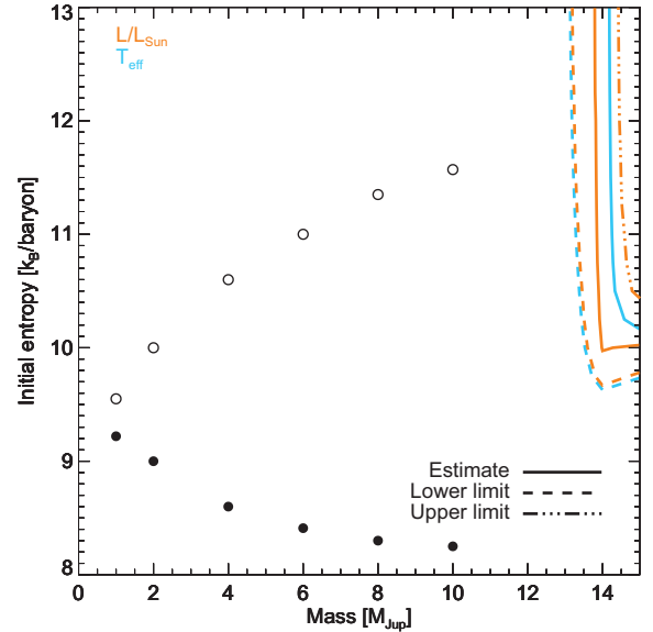
Fig. 11. Predictions of the “warm-start” evolutionary models of SB12 for \kappa And b for a system at t \approx 30^{+20}_{-10} Myr. The extreme values of the companion age, T_{\text{eff}} , and luminosities define a range of masses and initial entropies lying between the dashed and dotted-dashed curves. We also overlay the initial entropies considered in “hot-start” (open circles) and “cold-start” (dots) models of FM08 (based on Marley et al. 2007).
