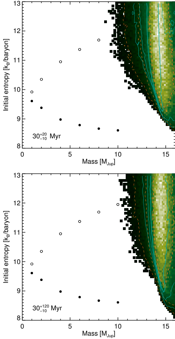
Fig. 12. Joint posteriors on the mass and initial entropy of \kappa And b obtained through MCMC runs with the models of Marleau & Cumming (2013), which include deuterium burning, from T_{\text{eff}} (solid lines) and the bolometric luminosity (dashed lines) of \kappa And b, assuming Gaussian errorbars. Entropy values need to be decreased by 0.45 k_{\text{B}}/\text{baryon} when comparing with SB12. The contours indicate the 68-, 95- and 99 % confidence levels (thick to thin lines). The colour (from dark to light) is proportional to the joint posterior probability at each M and S_{\text{init}} location in the T_{\text{eff}} -based run. The age was taken as t = 30^{+20}_{-10} Myr (top panel) and t = 30^{+120}_{-10} Myr (bottom panel).
