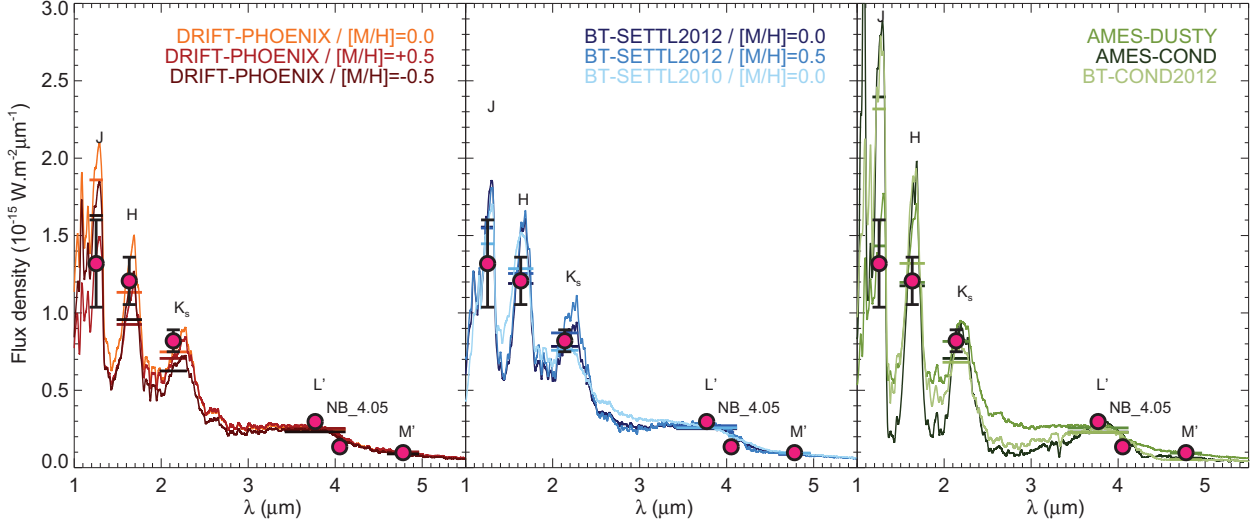
Fig. 8. Best fitted synthetic flux (horizontal bars) to the spectral-energy distribution of \kappa And b (magenta dots) considering the DRIFT-PHOENIX models with three different metallicities (left panel), the BT-SETTL models (middle panel), the AMES-DUSTY, AMES-COND, and BT-COND2012 models (right panel). The corresponding synthetic spectra are overlaid in each panel.
