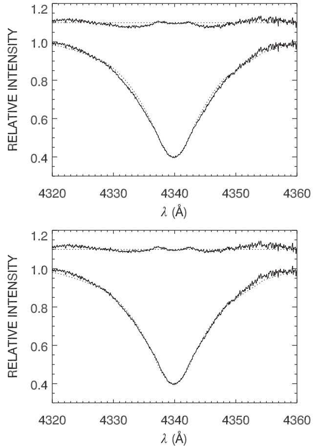
Fig. B.1. Hydrogen H \gamma line of \kappa And A (solid lines) fitted by atmospheric models (dotted lines). Residuals from the fit are shown in the upper part of the figures. Top: Solution where the line wings and the core are well fitted, but where the fit degrades in the line breadth. Bottom: Solution for which the line breadth is better fitted. These solutions were combined to derive the new estimate of the temperature and the surface gravity of the star.
