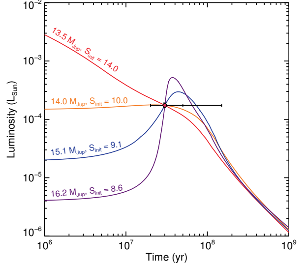
Fig. 13. Examples of possible cooling curves for \kappa And b using \log L/L_{\odot} = -3.76 at 30 Myr, with the corresponding mass and initial entropy (to be decreased by 0.45 k_{\text{B}}/\text{baryon} when comparing with SB12) of each curve indicated in the figure. For the lower entropies, we find that \kappa And b could be presently undergoing a deuterium ‘flash’ (Salpeter 1992; Bodenheimer et al. 2013, Marleau & Cumming, in prep.).
