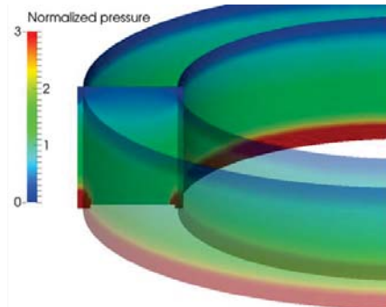
Figure 6. Normalized pressure distribution in the TDU thruster as predicted by the Direct Simulation Monte Carlo.
