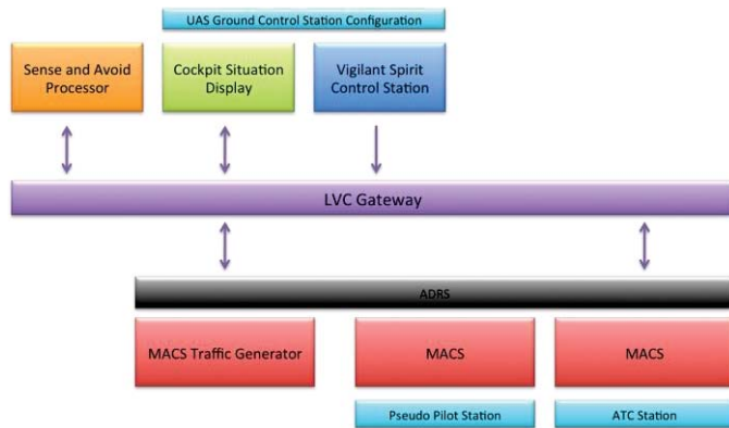
Figure 2. The simulation architecture used to support HSI HITL simulations with the prototype GCS.
