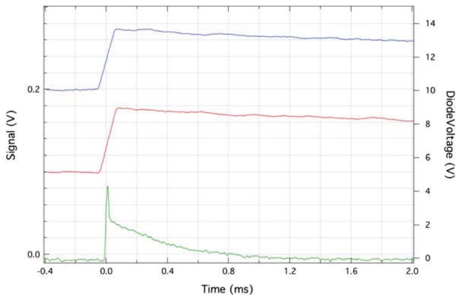
Fig. 4 Top 6 keV Mn K_{\alpha} X-ray, middle 6 keV diode pulse, bottom voltage pulse across the diode. The voltage pulse tail is below the threshold of the diode and contributed no light. The voltages are offset for comparison. The traces were DC coupled and triggered off of the detector signal. (Color figure online)
