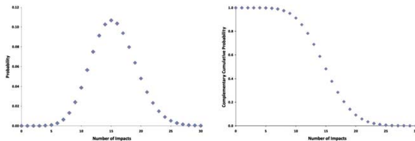
Figure 9. (left) Impact probability for polar locations, showing that 14–16 anomalous craters might be expected within \pm 20^\circ of the poles if they were not somehow correlated to the unique environment of the poles. Seventy-two polar anomalous craters and 88 nonpolar anomalous craters have been identified. (right) Complementary cumulative probability associated with Figure 9 (left). Values on the y axis indicate the probability of finding more than the number of impacts identified on the x axis. The probability of finding more than 30 anomalous impact craters in the polar regions due strictly to random processes is effectively zero ( <0.0001 ).
