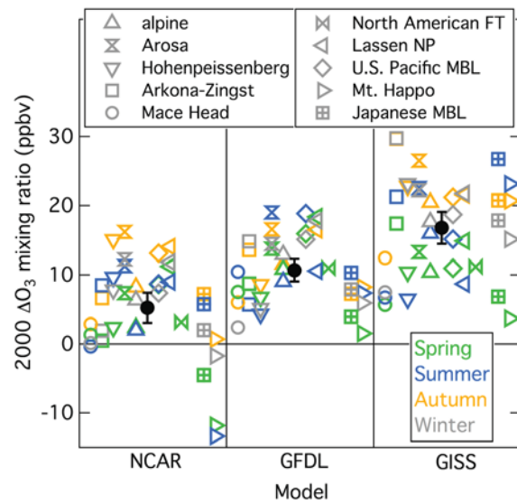
Figure 2. Difference between modeled and measured seasonally averaged year 2000 O 3 concentrations (ΔO 3 ) for five European (left of black symbols with error bars), three western North American (right of symbols), and two Asian data sets (far right in each panel). Data sets and seasons are indicated by different symbols and colors, respectively, as indicated in the annotations. The three panels compare results from the three indicated models. The black symbols indicate averages over all ten data sets for each of the models; the error bars give 2σ confidence limits of the averages.
