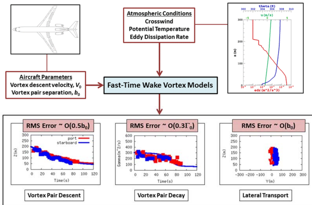
Figure 1. The flowchart shows the fast-time wake model inputs and outputs (MKS units). The average root mean square (RMS) errors in the model prediction of vortex circulation strength and location are also given.
