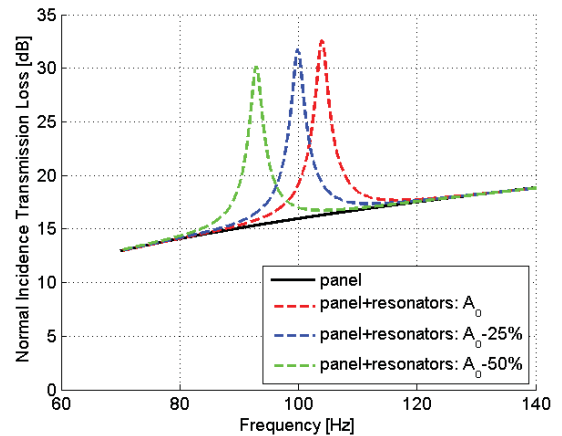
Figure 11: Effect of inlet area on transmission loss.
