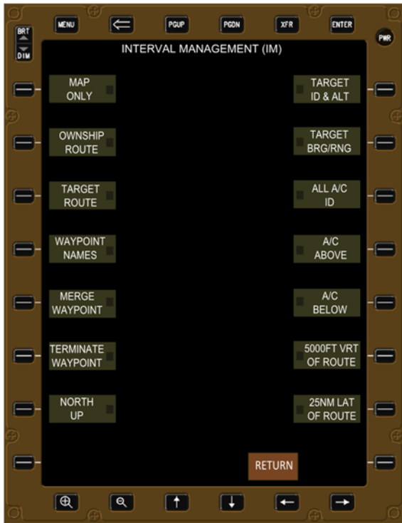
Figure D-2. No filters selected and corresponding display.
