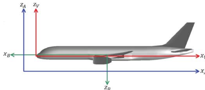
Figure 12. GTM Coordinate Systems
