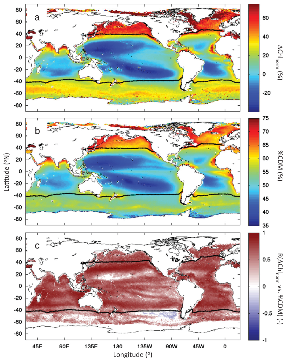
Fig. 5. The importance of CDM on retrieval of phytoplankton chlorophyll from satellite ocean color observations. a) The mission mean normalized chlorophyll concentration anomaly, \Delta\text{Chl}_{\text{norm}} . Values of \Delta\text{Chl}_{\text{norm}} are calculated as the normalized difference between \text{Chl}_{\text{OC4}} and \text{Chl}_{\text{GSM}} ( \Delta\text{Chl}_{\text{norm}} = 100 * (\text{Chl}_{\text{OC4}} - \text{Chl}_{\text{GSM}}) / \text{Chl}_{\text{GSM}} ; Siegel et al., 2005b). b) The mission mean fraction of non-water light absorption at 443 nm that can be attributed to CDM, %CDM (Siegel et al., 2005b). Values of %CDM are calculated as 100 * \text{CDM} / (\text{CDM} + a_{\text{ph}}(440; \text{Chl}_{\text{GSM}})) where a_{\text{ph}}(440; \text{Chl}_{\text{GSM}}) = 0.0378 (\text{Chl}_{\text{GSM}})^{0.627} (Bricaud et al., 1998). The Bricaud et al. (1998) a_{\text{ph}}(440) model is used in the %CDM definition because the GSM model was constructed to estimate values of \text{Chl}_{\text{GSM}} and not a_{\text{ph}}(440) (Maritorena et al., 2002). c) The regional-scale distribution of the correlation coefficient (R) for the relationship between \Delta\text{Chl}_{\text{norm}} and %CDM. Only significant (at the 95% c.i.) correlation values are plotted. The mean SST = 15 °C isotherm is shown as the black lines. This updates figures from Siegel et al. (2005a) and Siegel et al. (2005b) using the 2010.0 version of the SeaWiFS data set.
