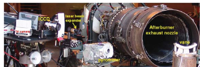
Figure 28.—Photographs of Cr:GAP-coated Honeywell stator vane doublet positioned aft of the J85 engine afterburner exhaust nozzle. ICCD, laser beam expander, and 8- \mu m pyrometer are aligned to focus on the same region of the vane surface.
