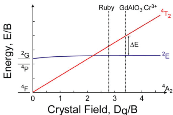
Figure 2.—Tanabe-Sugano diagram showing relationship between 4 T 2 and 2 E energy levels and crystal field for Cr 3+ 3d 3 electron configuration. Dotted lines show that higher crystal field in Cr:GAP will lead to substantially higher energy difference between these levels compared to ruby.
