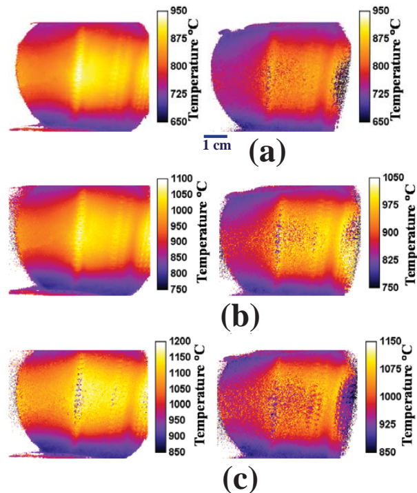
Figure 27.—Comparison of surface temperature maps of left-hand vane in burner rig flame without (left) and with (right) rust stain deposit on vane surface. No cooling air flow. (a) low, (b) middle, and (c) high burner flame setting.
