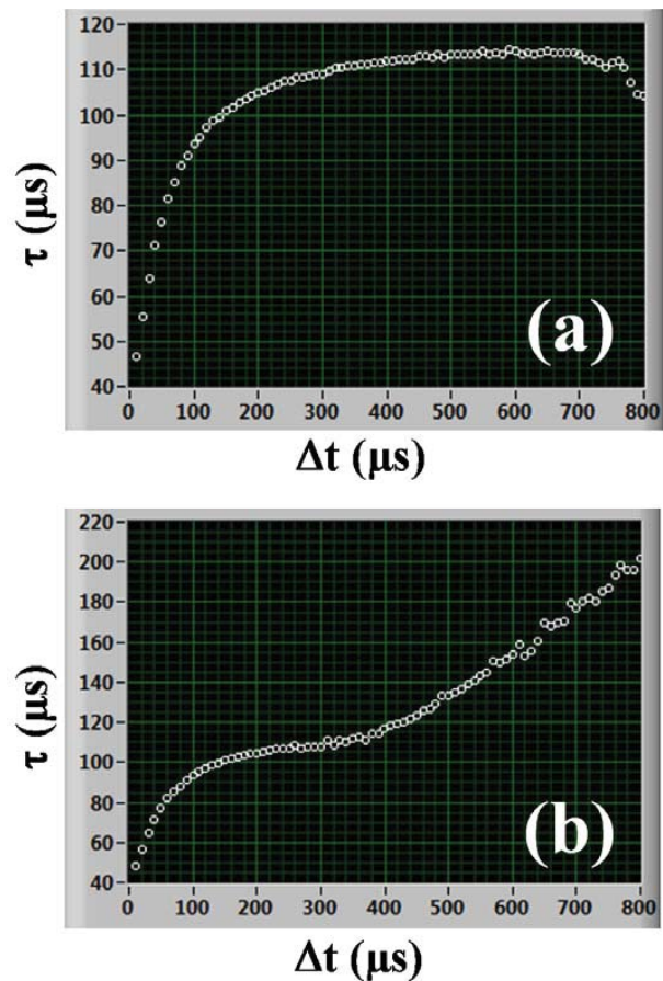
Figure 16.—Effect of dual gate selection on estimated single decay constant, \tau , obtained from simulated biexponential decay with \tau_1 = 20 \mu\text{s} and \tau_2 = 120 \mu\text{s} . Initial gate delay is fixed at start of decay and \Delta t is time interval between first gate delay and second gate delay. (a) No background noise included in simulation. (b) Background noise included in simulation.
