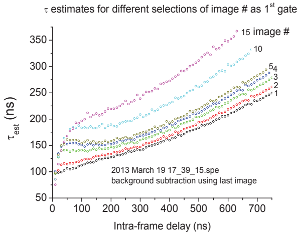
Figure 17.—Estimates of decay time, \tau_{est} , determined from different dual gate delay selection times from luminescence images of a 25.4 mm diameter specimen heated by CO 2 laser to uniform temperature of 1250 °C. Each curve represents selection of specific initial gate delay time with each point in the curve representing choice of the second gate delay time. Each curve number increment corresponds to selecting the initial gate delay 10 ns later than the previous curve number, starting with an initial gate delay of 45 ns for curve 1.
