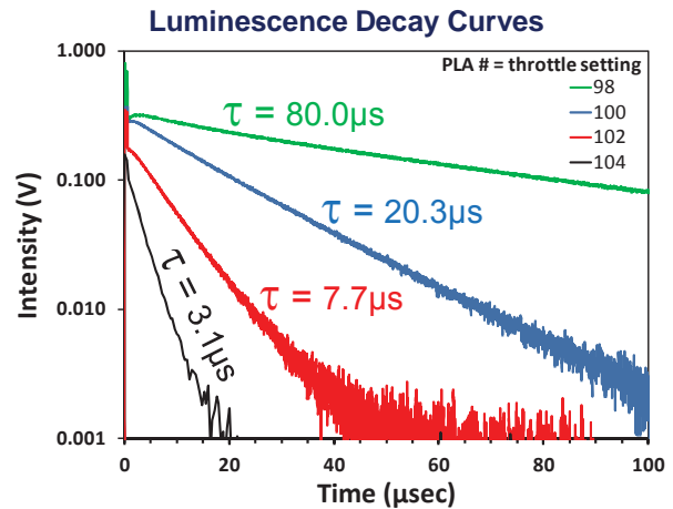
Figure 9.—Luminescence decay curves acquired from Cr:GAP-coated vane at different throttle settings of J85 test engine at UTSI.
