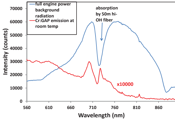
Figure 33.—Spectral plot comparing intensity of the thermal background collected by engine probe at full engine power with luminescence emission intensity collected from Cr:GAP-coated vane surface at room temperature using same engine probe. Note that emission from the Cr:GAP phosphor has been multiplied by a factor of 10000 in order to be discernible.
