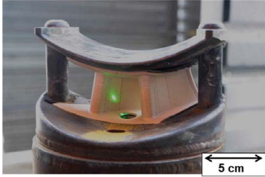
Figure 6.—Honeywell stator vane in AEDC test fixture. Green spot is excitation laser showing location of temperature measurement.
