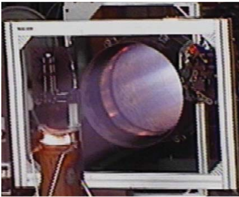
Figure 7.—Aft view of Cr:GAP-coated Honeywell stator vane doublet in afterburner flame of J85 test engine at UTSI.
