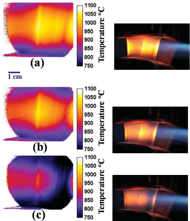
Figure 23.—Surface temperature maps of left-hand vane in burner rig flame at medium burner flame setting over range of cooling air flow settings: (a) 0 psi, (b) 10 psi, and (c) 20 psi cooling flow control pressure. Maps produced from 64-gate-delay sequences, 10 delay sequences averaged. (a) and (b) 8 on-chip accumulation repeats for each gate delay, gate delay increment = gate width = 1.25 \mu s; (c) 4 on-chip accumulation repeats for each gate delay, gate delay increment = gate width = 2.5 \mu s. Photographs are of stator vane doublet in burner rig flame at corresponding cooling air flows.
