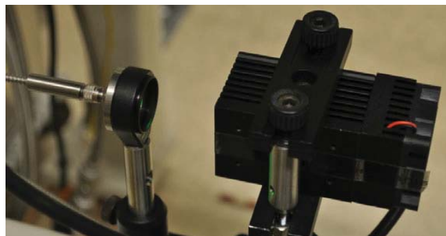
Figure 30.—Compact 532 nm laser diode positioned to couple into excitation fiber optic leg of engine probe.
