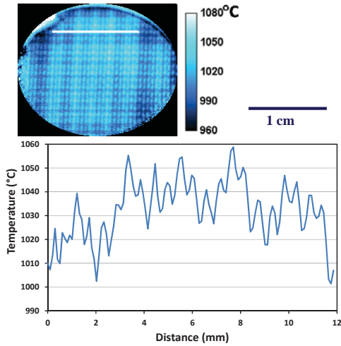
Figure 13.—(top) 2D temperature map of thermal test pattern at heat flux #1. Map produced from 20-gate-delay sequence, 10 repeats for each gate delay, gate delay increment = gate width = 0.5 \mu s. (bottom) Temperature line scan corresponding to white line.
