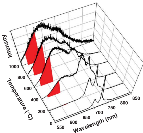
Figure 3.—Temperature dependence of luminescence emission spectra for Cr:GAP. Excitation at 532 nm. Red-shaded regions show wavelength range corresponding to bandpass selected for luminescence decay measurements.
