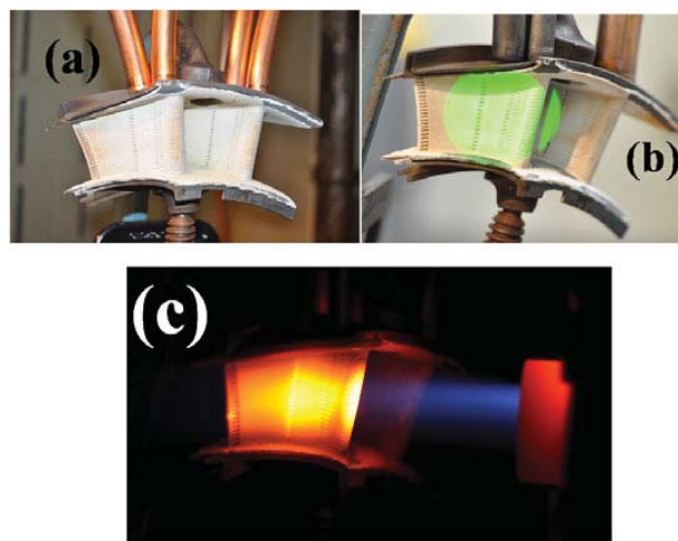
Figure 21.—(a) Photograph of Cr:GAP-coated Honeywell stator vane doublet showing copper tubing used to force air through the vane's cooling hole. (b) Broadened excitation laser beam (532 nm wavelength) illuminating area of interest near leading edge of left-hand vane. (c) Photograph of stator vane doublet positioned in high gas flow flame of NASA GRC Mach 0.3 burner rig facility.
