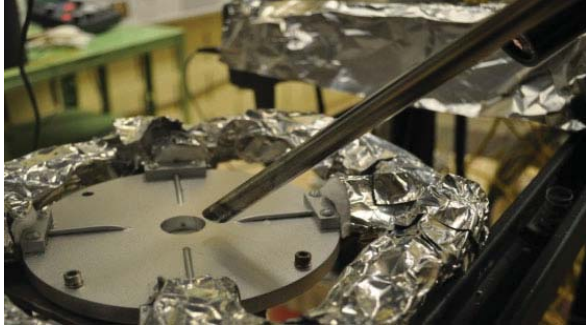
Figure 31.—Sensing end of engine probe positioned above high heat flux laser facility mounting stage.
