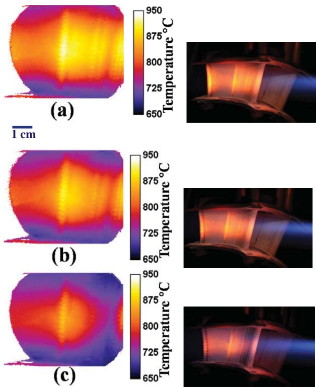
Figure 22.—Surface temperature maps of left-hand vane in burner rig flame at low burner flame setting over range of cooling air flow settings: (a) 0 psi, (b) 10 psi, and (c) 20 psi cooling flow control pressure. Maps produced from 64-gate-delay sequences, 2 on-chip accumulation repeats for each gate delay, gate delay increment = gate width = 7.5 \mu s. 10 delay sequences averaged. Photographs are of stator vane doublet in burner rig flame at corresponding cooling air flows.
