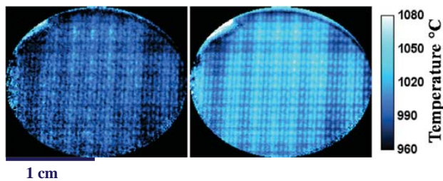
Figure 18.—The 2D temperature maps of thermal test pattern observed in Figure 13 obtained by (a) dual gate (2 and 5 \mu s gate delays) and multigate (20) decay time determination.
