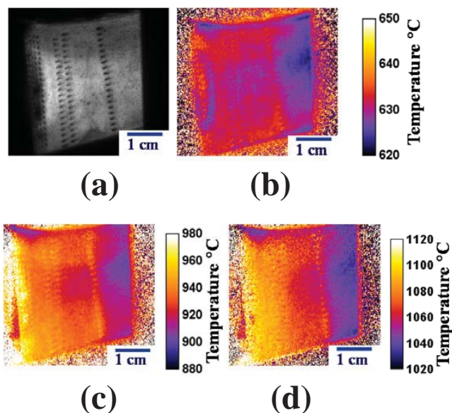
Figure 29.—Surface temperature maps of Honeywell stator vane exposed to afterburner flame of J85 test engine at UTSI with cooling air flow through cooling holes. (a) Field of view for temperature mapping. Temperature maps at different afterburner throttle settings. (b) PLA = 90. Map produced from 64-gate-delay sequences, 10 on-chip accumulation repeats for each gate delay, gate delay increment = gate width = 25 \mu s. 10 delay sequences averaged. (c) PLA = 99. Map produced from 16-gate-delay sequences, 20 on-chip accumulation repeats for each gate delay, gate delay increment = gate width = 2 \mu s. 8 delay sequences averaged. (d) PLA = 101. Map produced from 8-gate-delay sequences, 20 on-chip accumulation repeats for each gate delay, gate delay increment = gate width = 1 \mu s. 8 delay sequences averaged.
