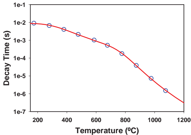
Figure 5.—Temperature dependence of Cr:GAP luminescence decay time for wavelengths selected by bandpass filter centered at 590 nm with a full-width half-max of 40 nm. Circles are values determined from measurements. Solid line is obtained by fitting Equation (1) to the data.
