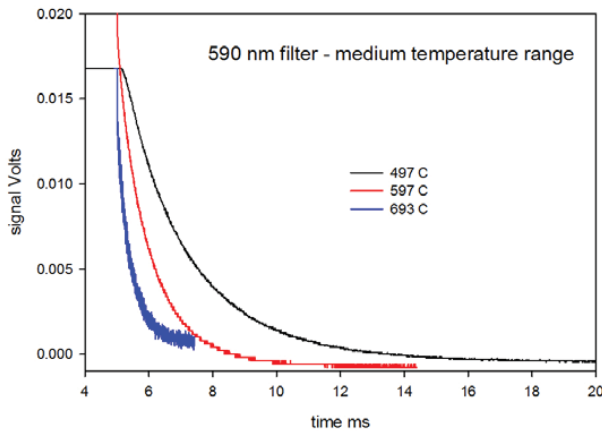
Figure 32.—Luminescence decay curves obtained from 500 to 700 °C from Cr:GAP-coated specimen using low power laser diode.
