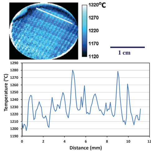
Figure 15.—(top) 2D temperature map of thermal test pattern at heat flux #3. Map produced from 20-gate-delay sequence, 10 repeats for each gate delay, gate delay increment = gate width = 0.1 \mu s. (bottom) Temperature line scan corresponding to white line.
