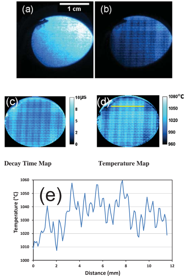
Figure 12.—2D temperature map construction for thermal “test pattern.” Background-corrected luminescence images obtained 0.5 \mu\text{s} (a) and 5.0 \mu\text{s} (b) after laser pulse. (c) Luminescence decay time map. (d) 2D temperature map. (e) Temperature line scan corresponding to yellow line in (d).
