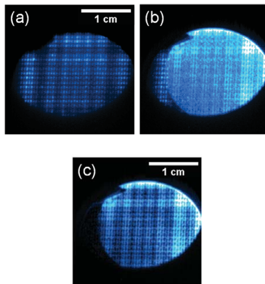
Figure 11.—Background subtraction for luminescence images of thermal "test pattern" produced by CO 2 laser heating of surface of Cr:GAP-coated disk. (a) Background image with no laser excitation. (b) Luminescence image obtained 16 \mu s after laser pulse without background subtraction. (c) Same luminescence image after background subtraction.
