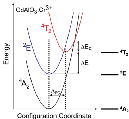
Figure 1.—Single configurational coordinate plot (left) and energy level diagram (right) for high-crystal-field Cr 3+ -doped phosphors such as Cr:GAP.
