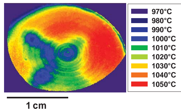
Figure 20.—The 2D temperature map of laser-heated Cr:GAP-coated disk subjected to crossed cooling air jets. Map produced from 8-gate-delay sequence, 10 repeats for each gate delay, gate delay increment = gate width = 3.0 \mu s.
