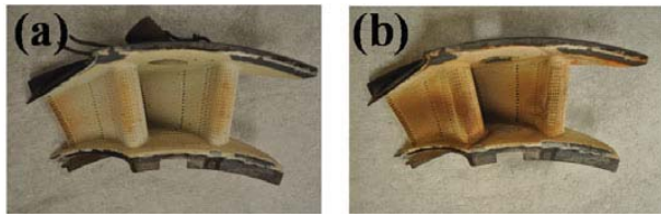
Figure 26.—Photographs of Cr:GAP-coated Honeywell stator vane doublet before (a) and after (b) rust deposition due to burner rig exposure.
