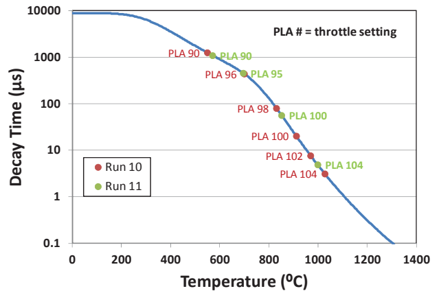
Figure 10.—Temperatures determined from luminescence decay time for Cr:GAP-coated vane at different throttle settings of J85 test engine at UTSI. Blue curve shows calibration between decay time and temperature.
