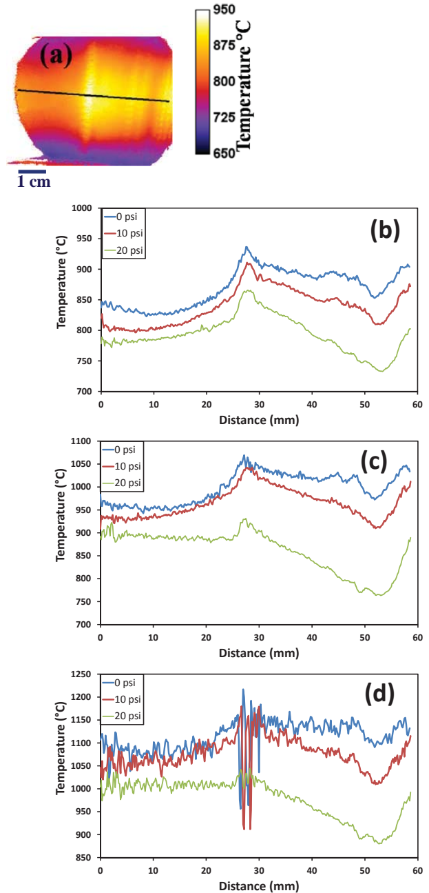
Figure 25.—Temperature line scans across temperature maps of vane in burner flame. (a) Black line indicates location of line scan traversing from left (downstream) to right (upstream) for condition of low burner flame setting and 0 psi cooling flow control pressure. Line scans from other temperature maps shown below are from same location. (b) Temperature line scans at low burner flame setting and three cooling flow levels. (c) Temperature line scans at medium burner flame setting and same three cooling flow levels. (d) Temperature line scans at high burner flame setting and same three cooling flow levels.
