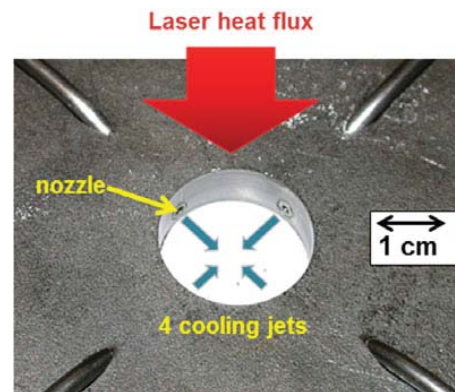
Figure 19.—Cooling air jet fixture for high heat flux laser heating facility.
