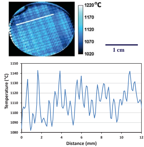
Figure 14.—(top) 2D temperature map of thermal test pattern at heat flux #2. Map produced from 20-gate-delay sequence, 10 repeats for each gate delay, gate delay increment = gate width = 0.5 \mu s. (bottom) Temperature line scan corresponding to white line.
