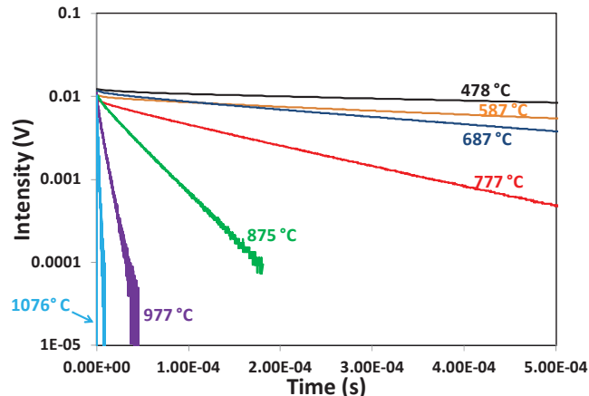
Figure 4.—Luminescence decay at various temperatures from Cr:GAP, using bandpass filter centered at 590 nm with a full-width half-max of 40 nm.
