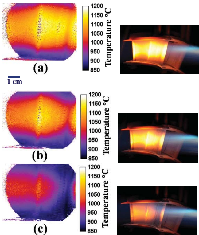
Figure 24.—Surface temperature maps of left-hand vane in burner rig flame at high burner flame setting over range of cooling air flow settings: (a) 0 psi, (b) 10 psi, and (c) 20 psi cooling flow control pressure. Maps produced from 32-gate-delay sequences, 8 on-chip accumulation repeats for each gate delay, gate delay increment = gate width = 0.625 \mu s. 10 delay sequences averaged. Photographs are of stator vane doublet in burner rig flame at corresponding cooling air flows.
