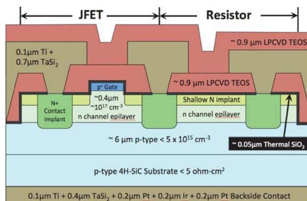
Fig. 1. Simplified cross-sectional schematic of NASA Glenn 4H-SiC JFET and resistor (sharing common n-type layer mesa).
