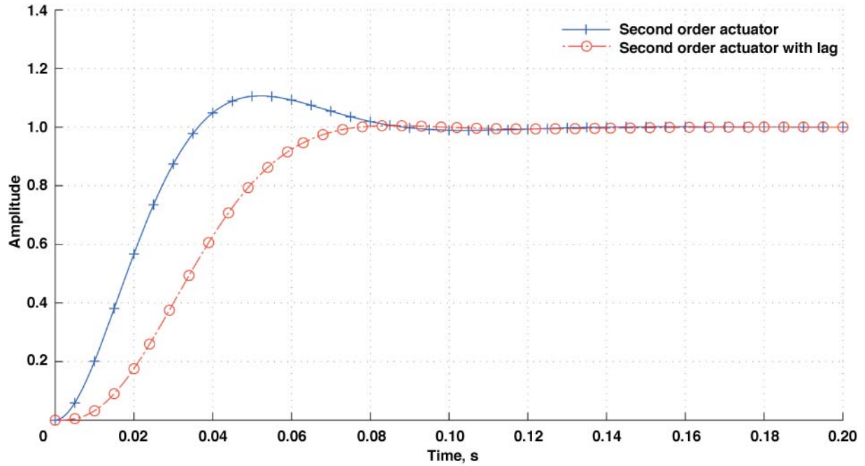
Figure 2. Actuator model.
