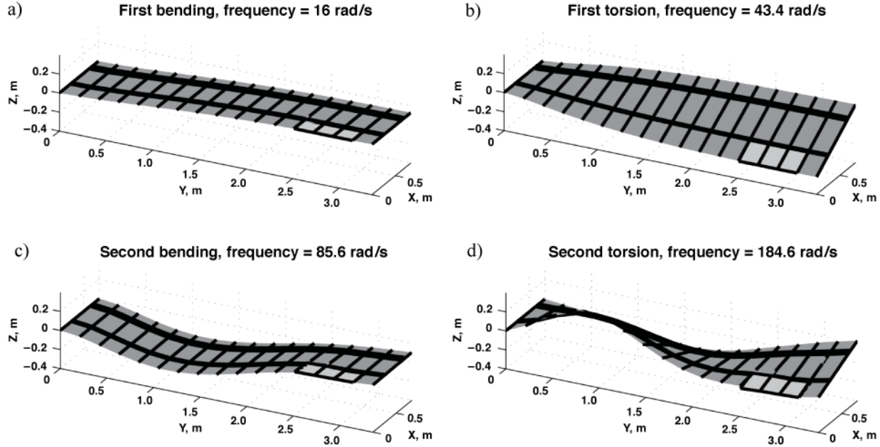
Figure 9. Modal Representation of wing model: a) 1 st bending; b) 1 st torsion; c) 2 nd bending; and d) 2 nd torsion.
