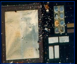
AO erosion of Kapton blanket
