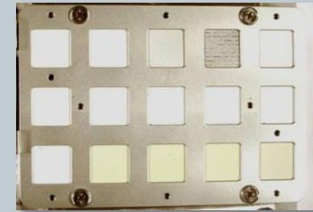
MISSE 6 Thermal Control Paints Experiment (post-flight)
