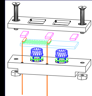
Exploded view drawing
