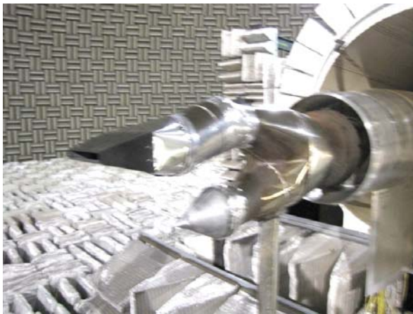
Figure 7 Blank-off plate and tapered closeout on lower leg of y-duct, used to obtain single-nozzle data (rectangular nozzle in this picture) on HFJER.
