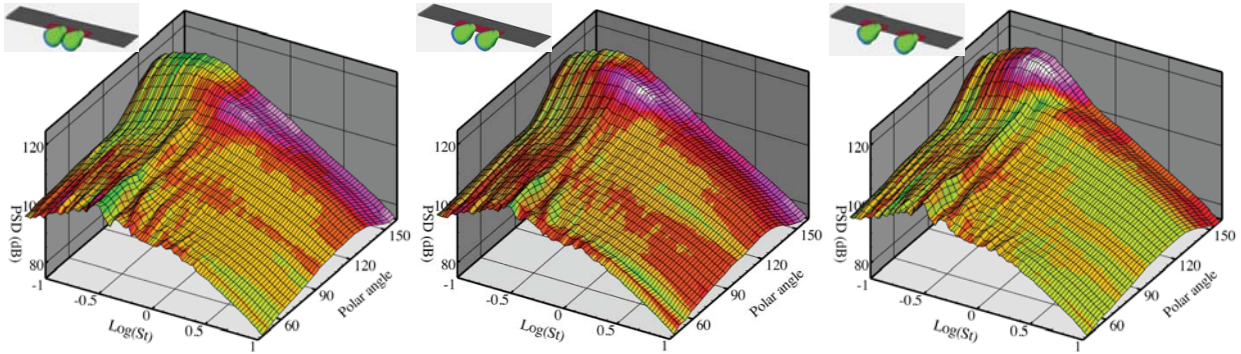
Figure 26 Same as Figure 25 except x_{TE} = 4'' .
