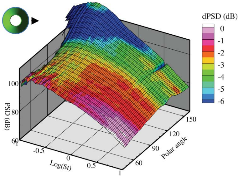
Figure 14 The effect of flight on spectral directivity of noise from a single round nozzle (TCO). Jet flow is Ma = 1.33 , T_{s,j}/T_{\infty} = 1.76 . Sound from jet in flight M_{flight} = 0.25 minus sound with no forward flight.
