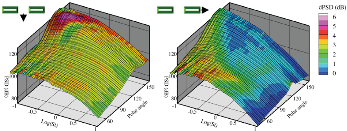
Figure 23 Same as Figure 22 except spacing s/D = 5.26 . Compare with Figure 20.
