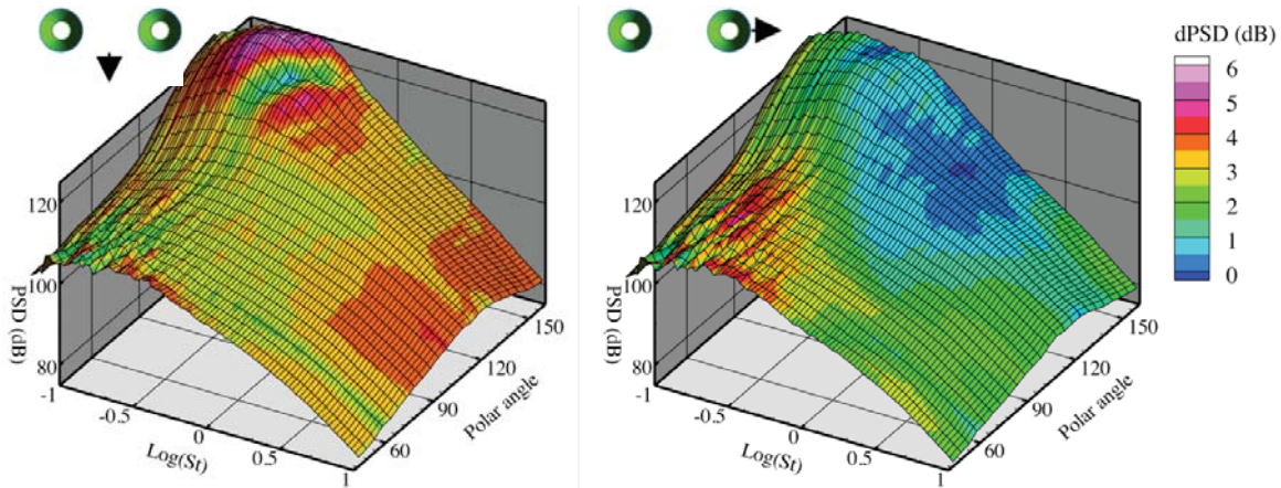
Figure 20 Same as Figure 19 except data from present tests and flow condition is Ma = 1.33 , T_{s,j}/T_\infty = 1.76 , M_{flight} = 0.1 .
