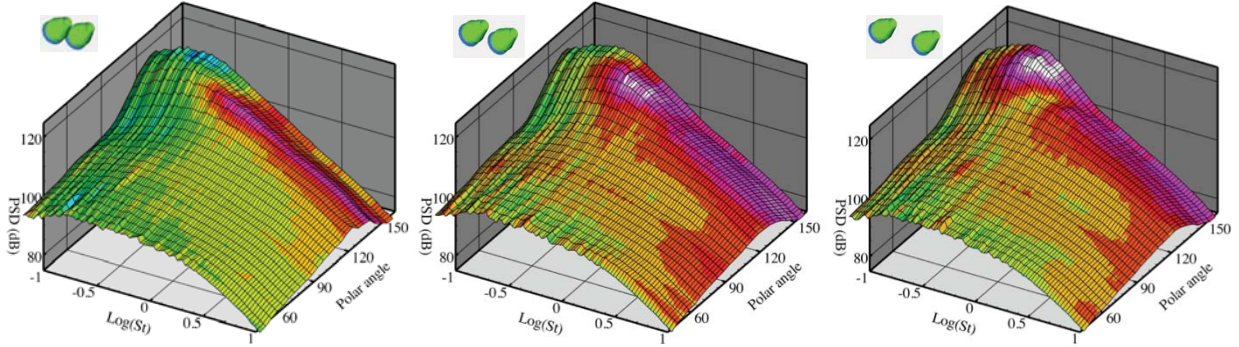
Figure 24 Difference in spectral directivity caused by adding a second jet in isolation (no surface). Plots are for different spacings (left to right: s/D = 2.62, 4.12, 5.62 ). Flow condition is unheated Ma = 0.9 , M_{flight} = 0 . Observer is in \phi = 0^\circ plane (normal to plane containing jet axes). Color scale spans from 0 to 6dB as in Figure 23.
