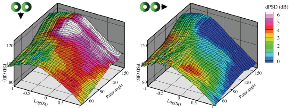
Figure 17 Difference in acoustic spectral directivity caused by adding a second round jet with spacing s/D = 2.62 as seen by observer normal to their common plane ( \phi = 0^\circ ; left) and in line with jets ( \phi = 90^\circ ; right). Shape is spectral directivity of two jets. Flow condition is Ma = 1.40 , T_{s,j}/T_\infty = 2.00 , M_{flight} = 0.1 .
