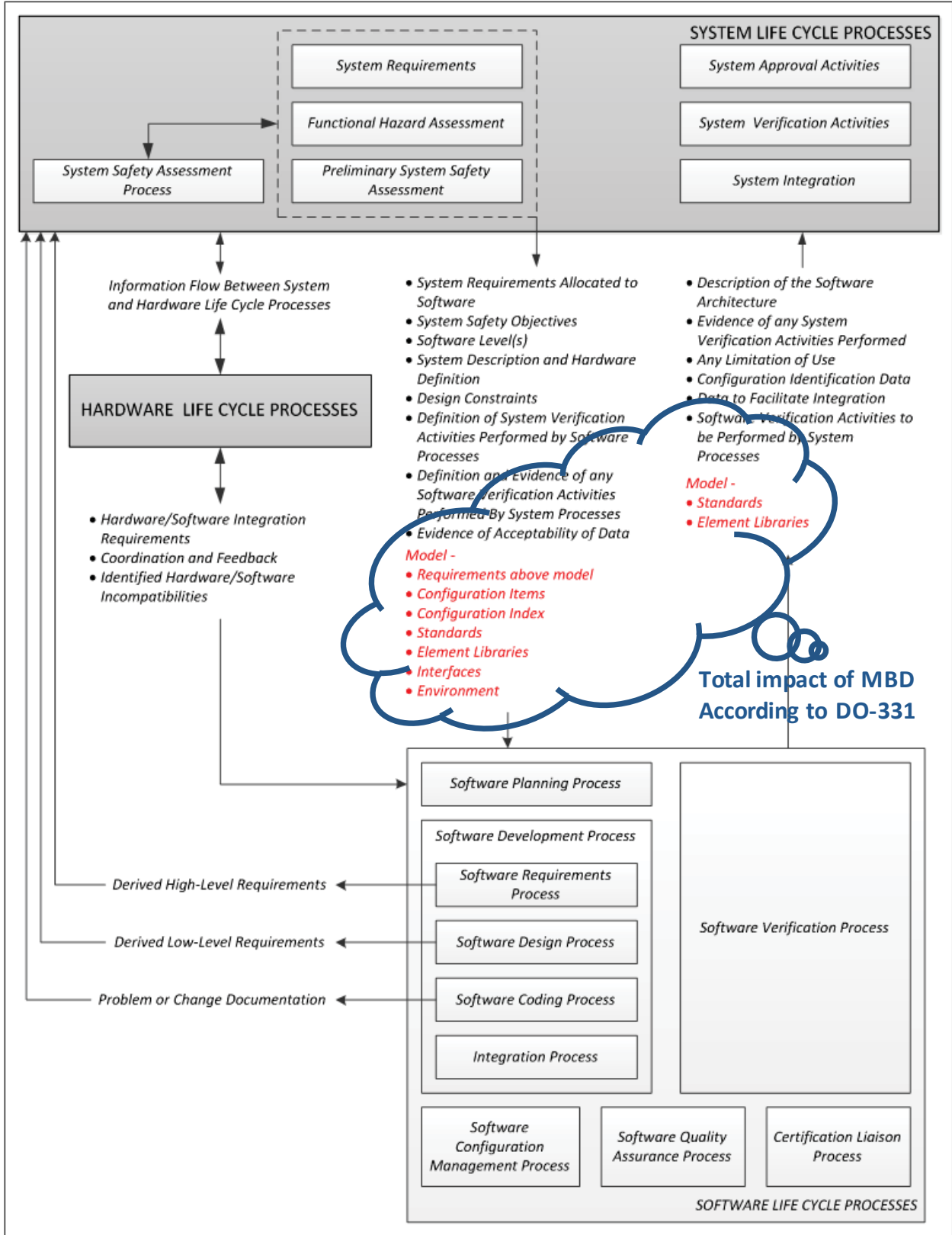
Figure 4. DO-331 MB.2-1
