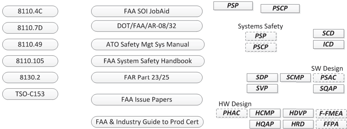
Figure 12. Document Forest
