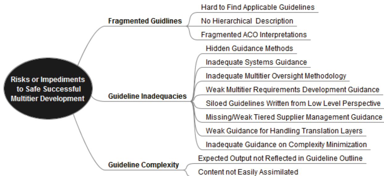
Figure 7. Guideline Weaknesses
