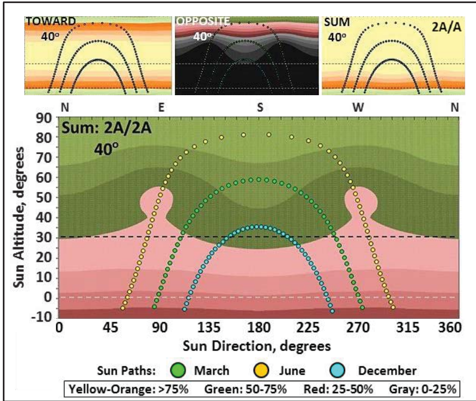
Figure 28. LTA solar energy collection contours: Santa Teresa, array mount angle = 40^\circ .
