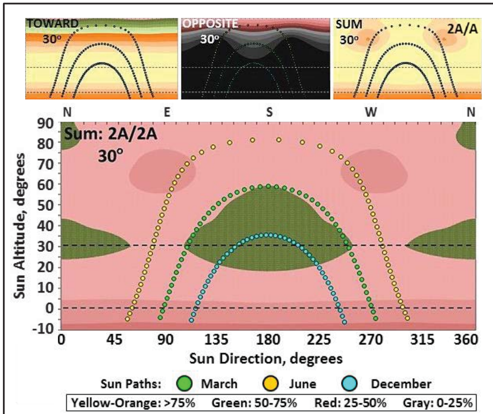
Figure 29. LTA solar energy collection contours: Santa Teresa, array mount angle = 30^\circ .
