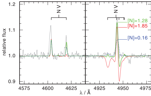
Fig. 22. Determination of the N abundance of K 1-27. N V lines in the EFOSC2 observation are compared with models with different N abundances as indicated by the labels.
