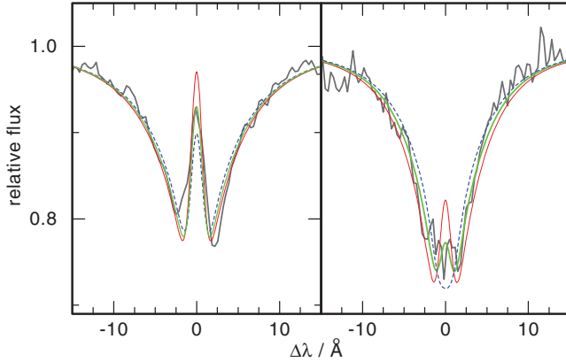
Fig. 16. Determination of T_{\text{eff}} of K 1–27 (left) and LoTr 4 (right) using the central emission of He II \lambda 4686 Å. The EFOC2 observation (solid black line) is compared with models with T_{\text{eff}} = 130/110 kK (dashed, blue), 135/120 kK (thick, green), and 140/130 kK (thin, red).
