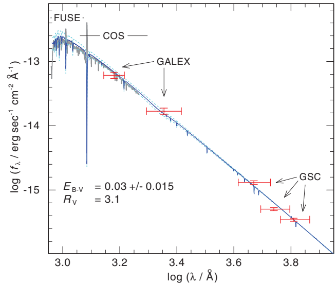
Fig. 15. Determination of E_{B-V} for HS 1522+6615. The FUSE and COS spectra and GALEX and BVR brightnesses from the GSC 2.3 catalog are used for comparison. The thick (blue) line is the spectrum of the final photospheric model. The dashed lines indicate the error limits.
