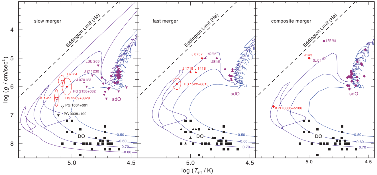
Fig. 26. Evolutionary tracks for a slow-merger ( left ), a fast-merger ( middle ) and a composite-merger ( right ) scenario of two He-WDs, marked with the merger mass in M_{\odot} (Zhang & Jeffery 2012b). The locations of the sdB-, sdO-stars, (purple, Müller-Ringat 2013; Németh et al. 2012; Naslim et al. 2010; Hirsch 2009; Ahmad et al. 2004; Rauch et al. 1998, 1991; Husfeld et al. 1989; Stroerer et al. 2007) and O(He) stars (red this work, Werner et al. 2014; Wassermann et al. 2010) as well as the DO WDs (black, Werner et al. 2014; Mahsereci 2011; Hügelmeier et al. 2006; Dreizler & Werner 1996) are marked. Open symbols indicate CSPNe, filled ones that no PN was detected. C-rich objects are represented by triangles, N-rich objects by inverted triangles, C- and N-rich objects by diamonds. Squares specify objects that are neither enriched in C nor in N.
