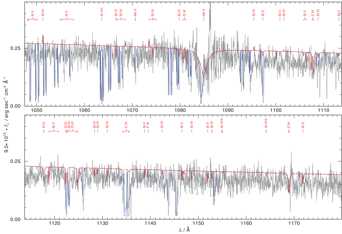
Fig. 3. Same as Fig. 1 for HS 1522+6615.
