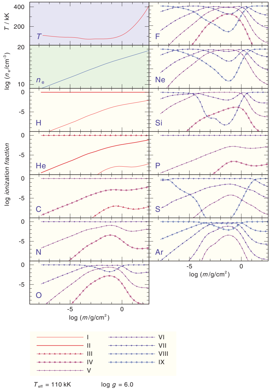
Fig. 12. Like Fig. 9, for HS 2209+8229.
