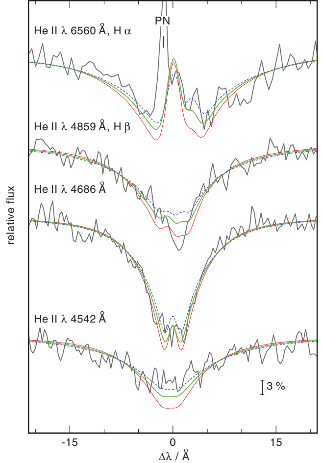
Fig. 17. Determination of \log g of LoTr 4. The EFOC2 observation (solid black line) is compared with models with \log g = 6.0 (dashed, blue), 5.8 (thick, green), and 5.6 (thin, red). The vertical bar indicates 3% of the continuum flux.
