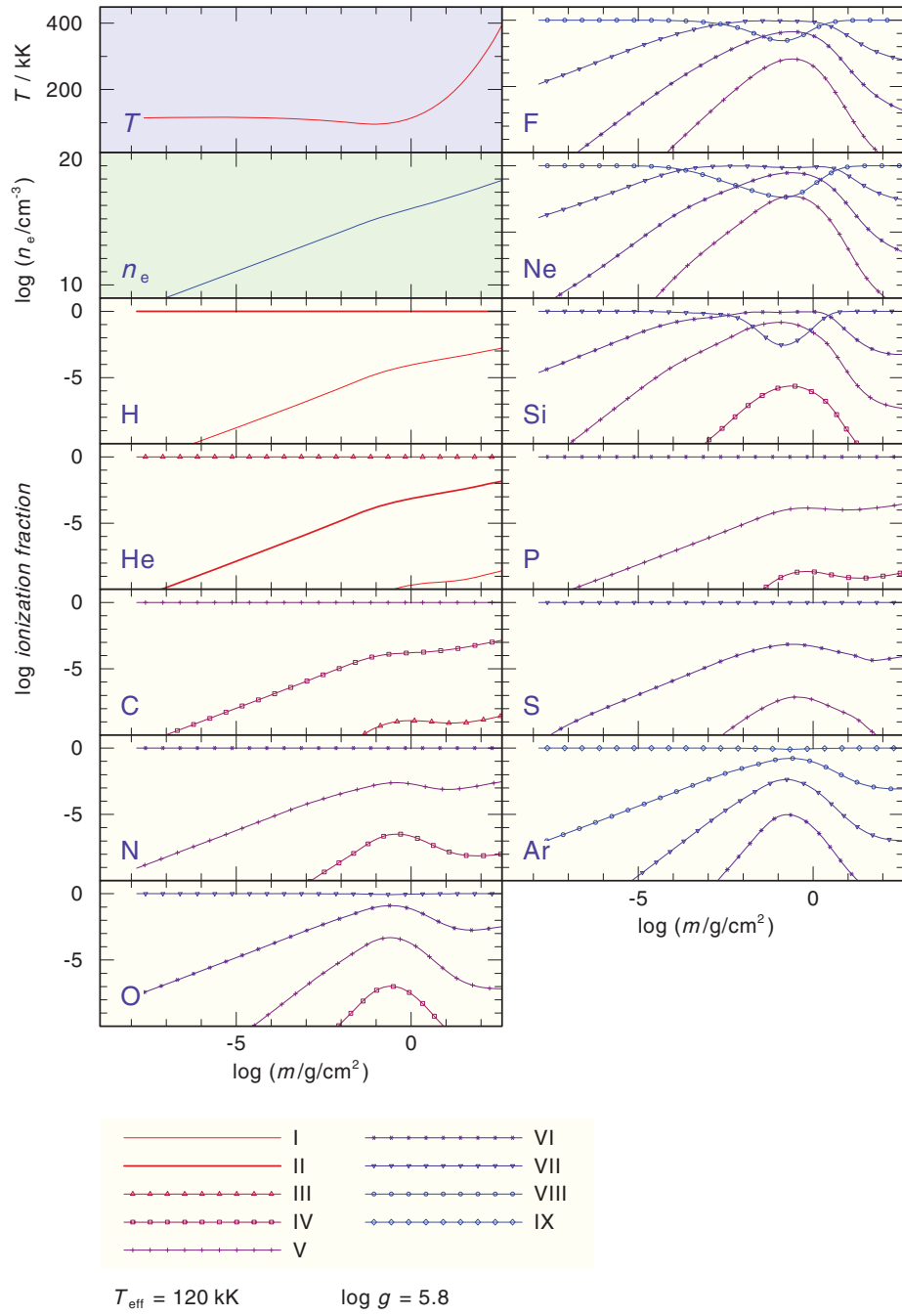
Fig. 10. Like Fig. 9, for LoTr 4.
