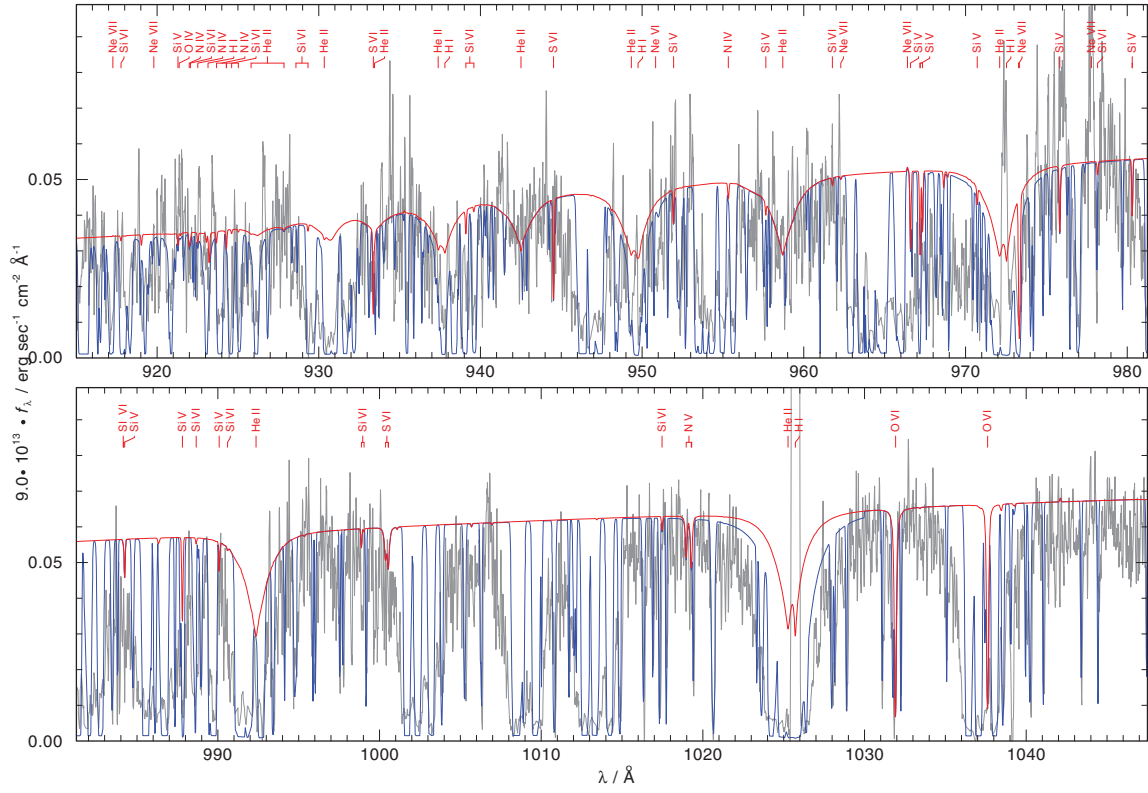
Fig. 2. Same as Fig. 1 for LoTr4.
