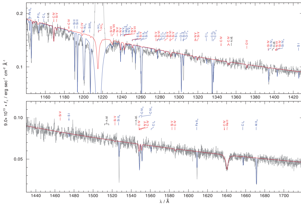
Fig. 7. Same as Fig. 5 for HS 1522+6615.
