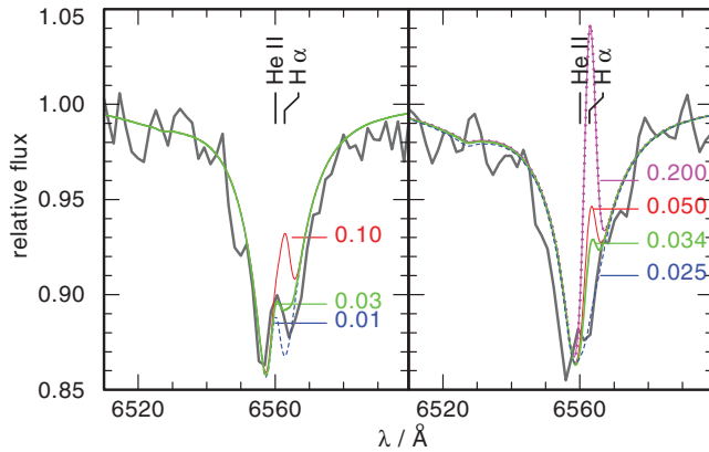
Fig. 19. Determination of the H/He ratio of HS 1522+6615 ( left panel ) and HS 2209+8229 ( right ). The observed H\alpha and He II line blend is compared with models with different H/He mass ratios, as indicated by the labels.
