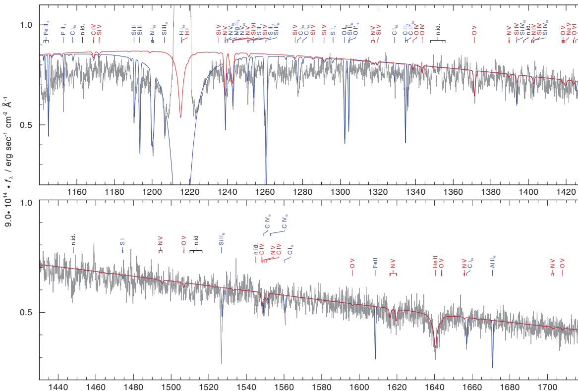
Fig. 8. Same as Fig. 5 for HS 2209+8229.
