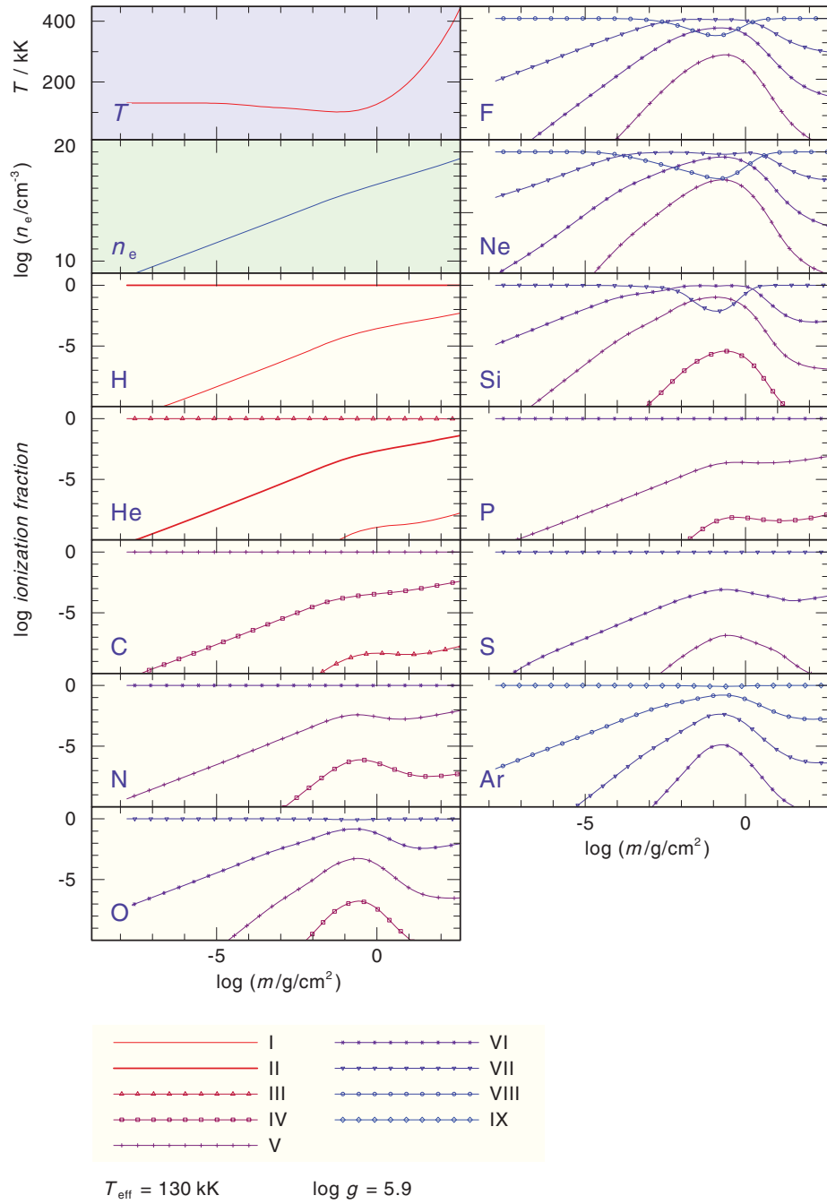
Fig. 11. Like Fig. 9, for HS 1522+6615.
