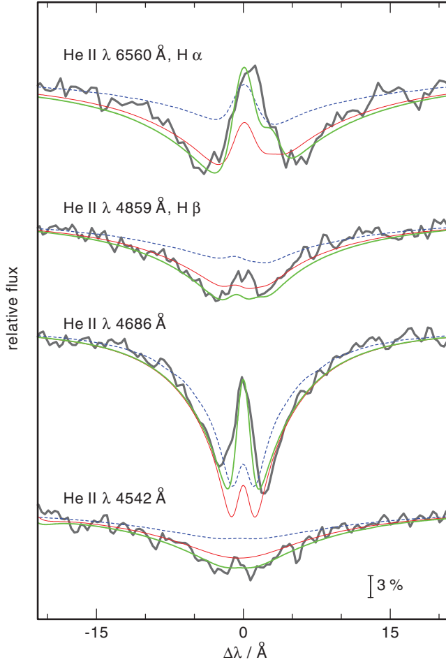
Fig. 13. Comparison of optical H I and He II lines calculated from models including H+He (dashed, blue), H+He+C+N+O (thin, red), and H+He+C+N+O+Ne (thick, green) with T_{\text{eff}} = 135 \text{ kK} and \log g = 6.4 , overplotted on the EFOSC2 spectrum of K 1–27. The vertical bar indicates 3% of the continuum flux.
