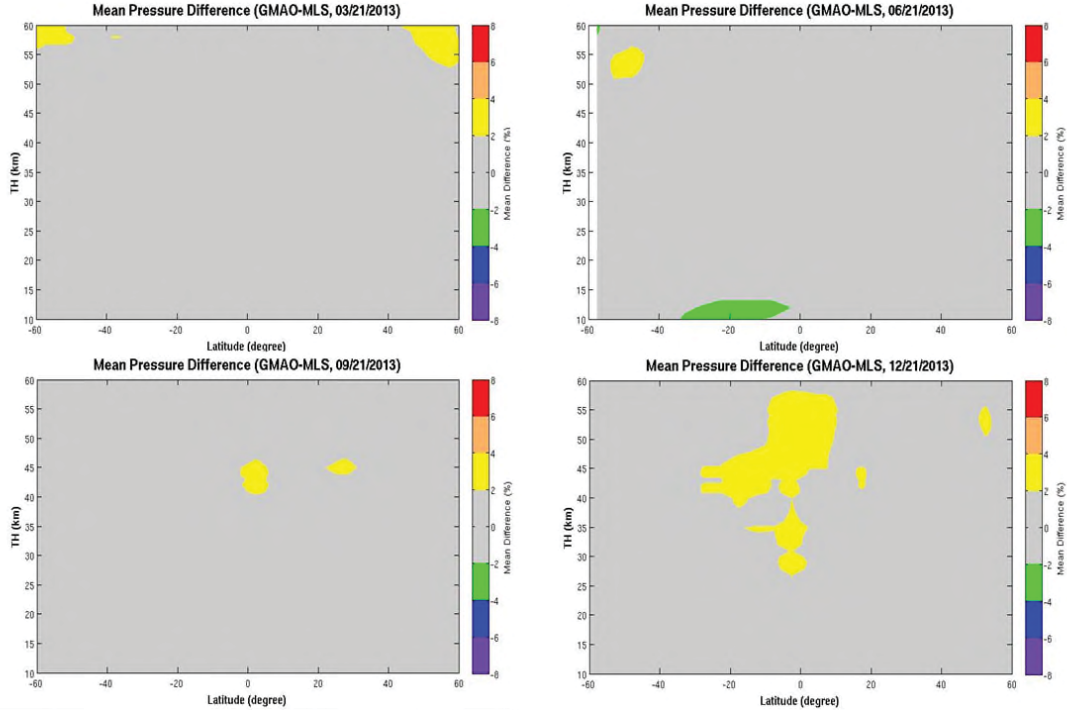
Figure 2: The daily zonal mean differences between GMAO and MLS pressure profiles. top left = March 21, top right = June 21, bottom left = September 21, bottom right = December 21. Gray areas indicate pressure differences less than \pm 2\% .
