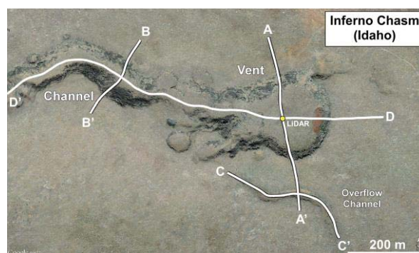
Figure 2. Location of Differential GPS and LiDAR surveys at Inferno Chasm in Idaho [GoogleEarth].
