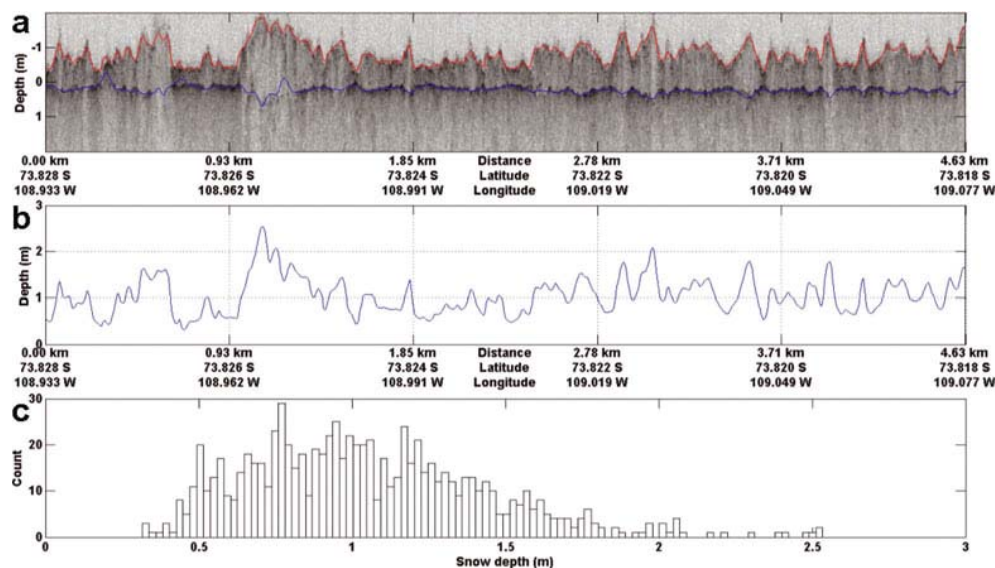
Fig. 9. Standard output from the interface tracker. (a) Extracted air/snow and snow/ice interfaces from the echogram presented in Figure 8. (b) Snow depth vs along-track position. (c) Histogram of snow thickness derived assuming a constant snow density of 0.3 \text{ g cm}^{-3} . Mean snow thickness for the segment was 93 cm.
