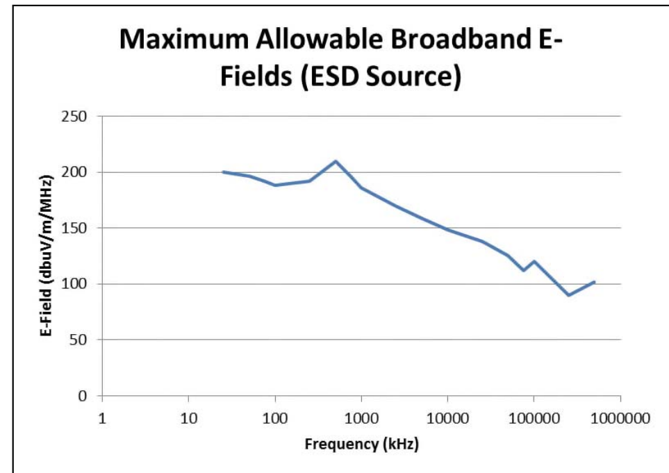
Sample broadband RF environment from EELV Specification. [3]
