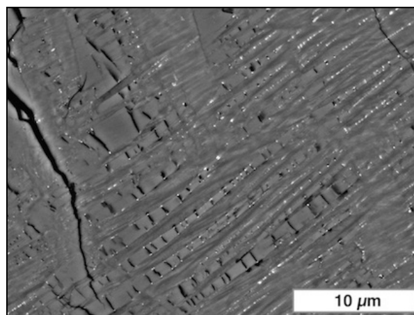
Fig. 1 BSE image of brown olivine in NWA 1950 showing a lenticular area with iron submicron-sized particles.
