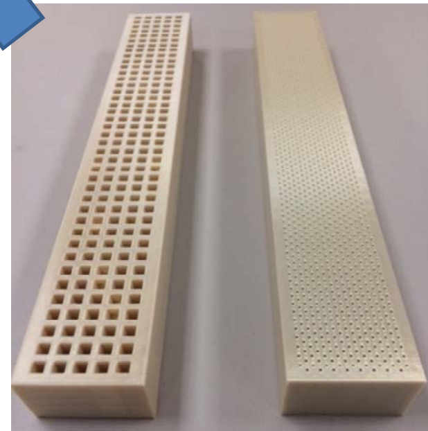
Baseline (right) and advanced liner test articles
