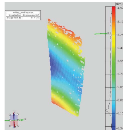
Digital Image Correlation Measurements
