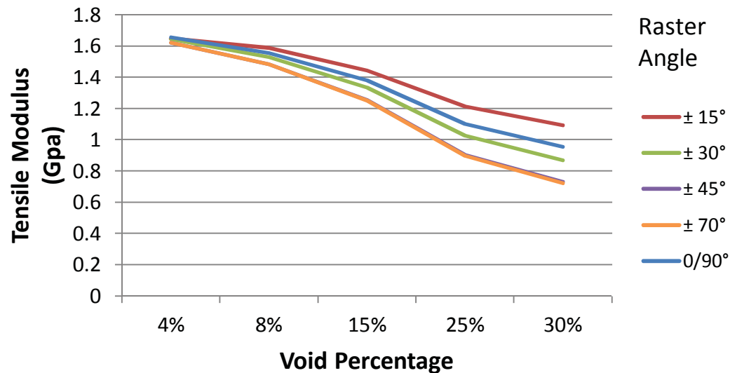
Tensile Modulus vs. Void Percentage at Varying Raster Angles
