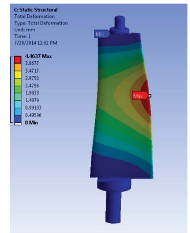
Finite Element Analysis
