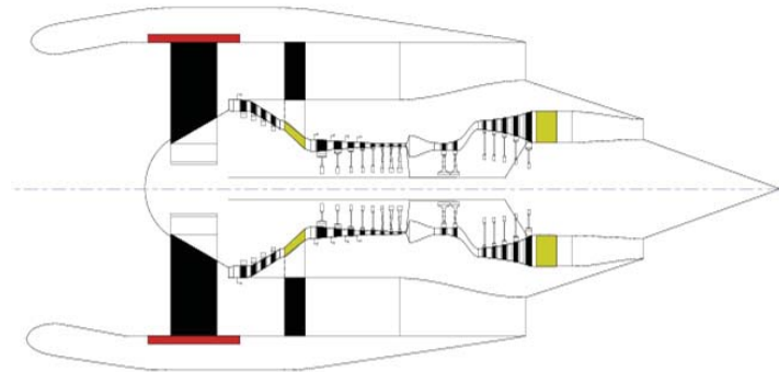
Model Propulsion system weight impacts (using WATE)
