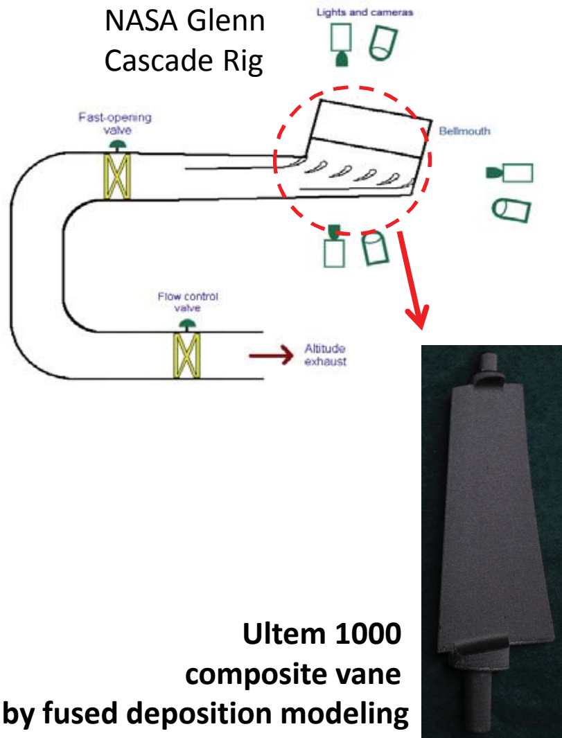
Vane Configuration in Cascade Rig
