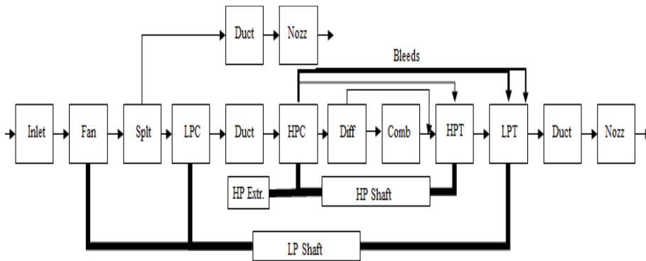
Model Propulsion system performance impacts (using NPSS)
